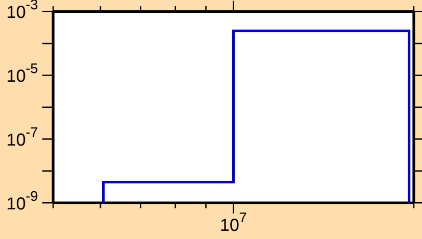
\sigma vs. E for ^{245}\text{Bk}(n,np)
