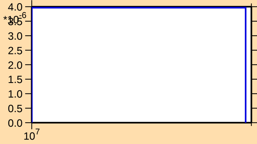
\sigma vs. E for ^{245}\text{Bk}(n,3n\alpha)
