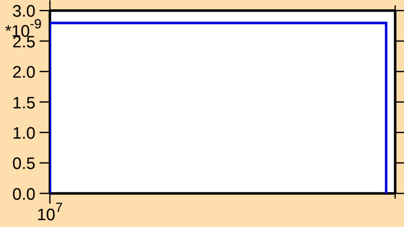
\sigma vs. E for ^{245}\text{Bk}(n,2np)
