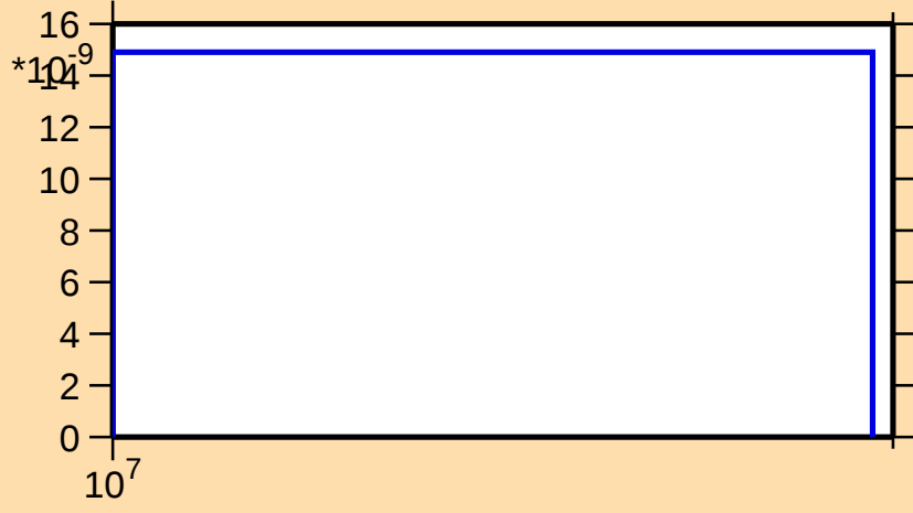
\sigma vs. E for ^{245}\text{Bk}(n,\text{nd})
