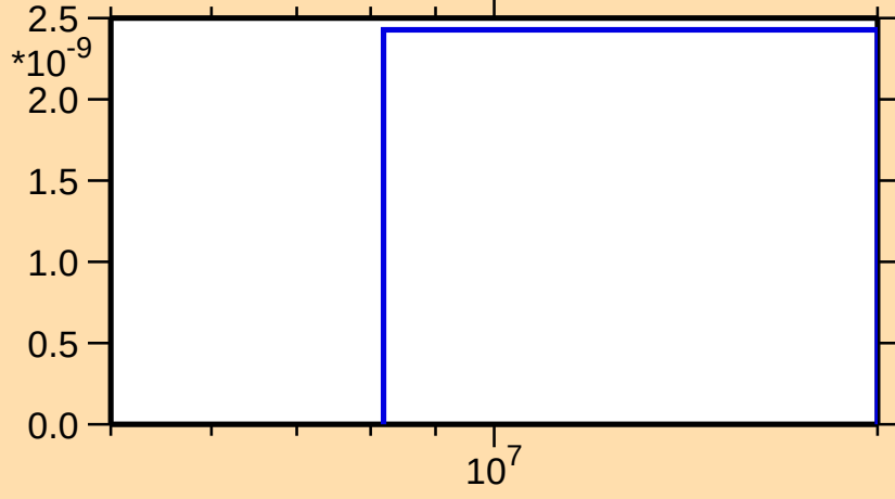
\sigma vs. E for ^{245}\text{Bk}(n,2np)
