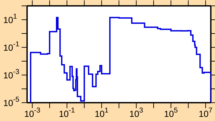
\sigma vs. E for ^{245}\text{Bk}(n,\gamma)
