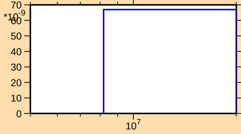
\sigma vs. E for ^{245}\text{Bk}(n,nt)
