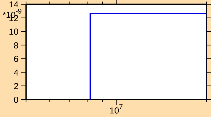
\sigma vs. E for ^{245}\text{Bk}(n,\text{nd})
