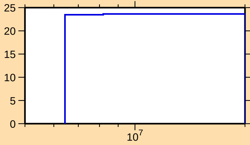
\Delta\sigma/\sigma vs. E for ^{245}\text{Bk}(n,\text{nonel.})
