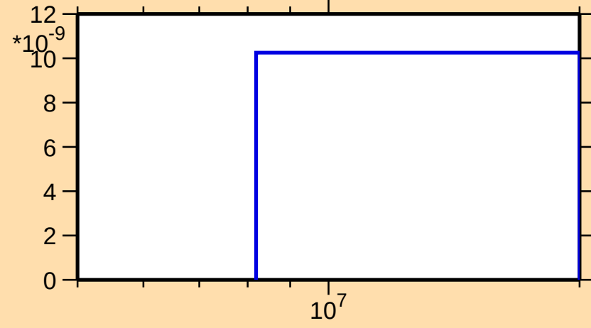
\sigma vs. E for ^{245}\text{Bk}(n,2n\alpha)
