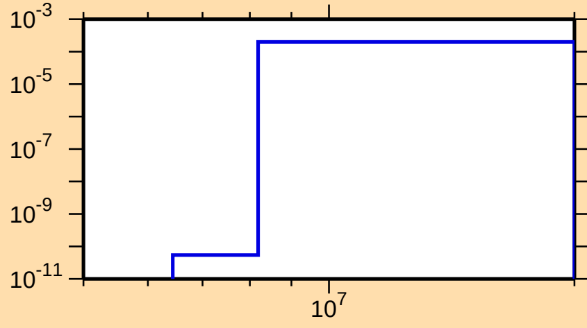
\sigma vs. E for ^{245}\text{Bk}(n,np)
