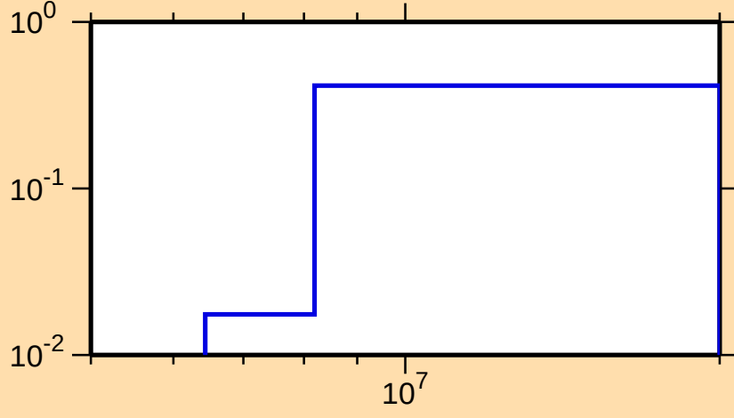
\sigma vs. E for ^{245}\text{Bk}(n,2n)
