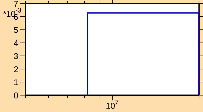
\sigma vs. E for ^{245}\text{Bk}(n,3n)
