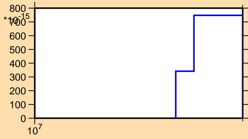
\sigma vs. E for ^{246}\text{Bk}(n,p\alpha)
