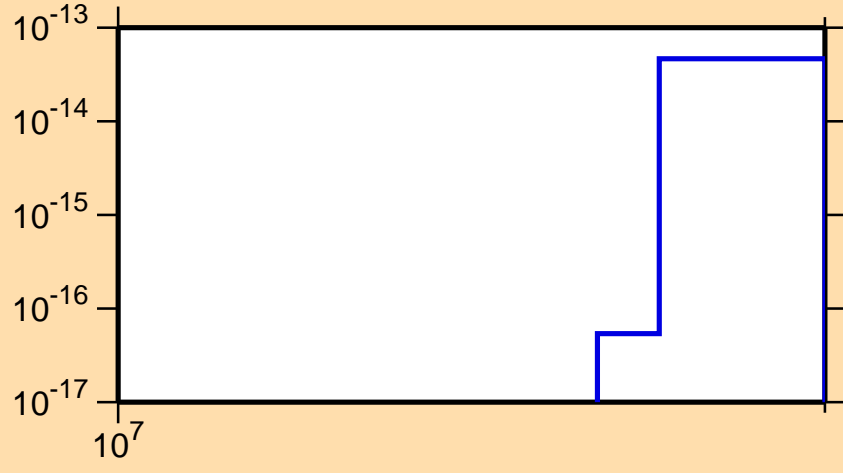
\sigma vs. E for ^{246}\text{Bk} (mt 34)
