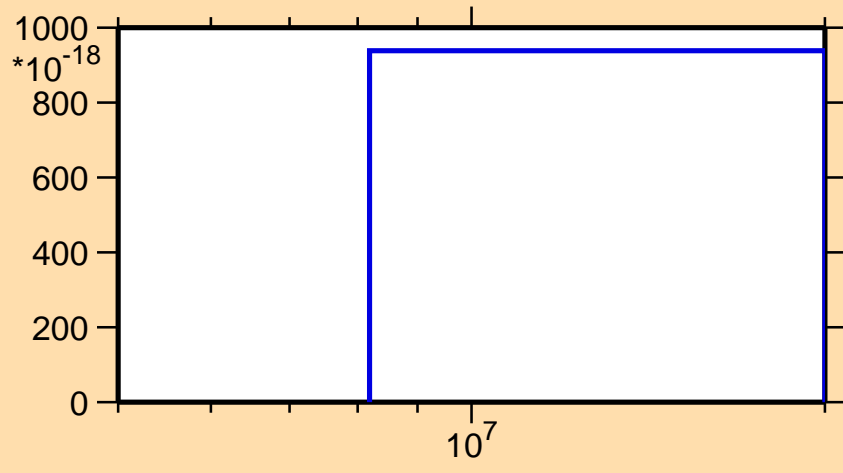
\sigma vs. E for ^{246}\text{Bk}(\text{mt } 11)
