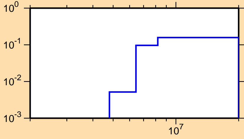
\sigma vs. E for ^{246}\text{Bk}(n,2n)
