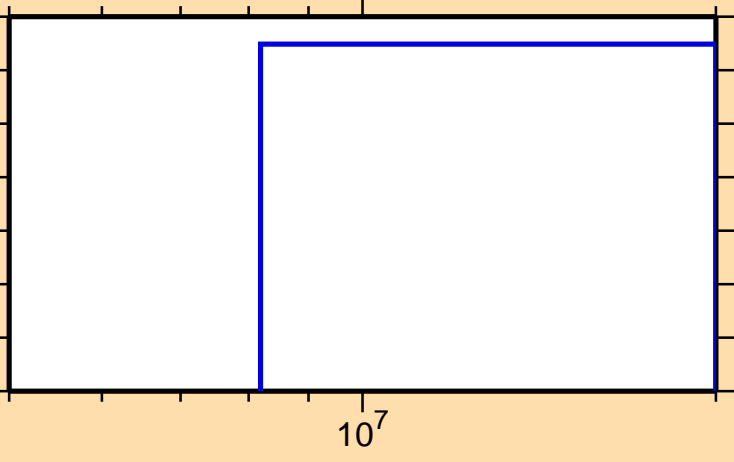
\sigma vs. E for ^{246}\text{Bk}(n,2np)
