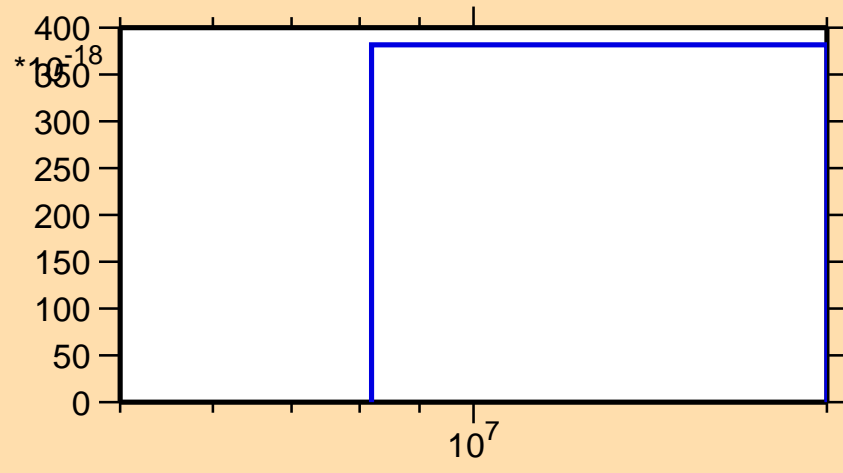
\sigma vs. E for ^{246}\text{Bk}(\text{mt } 34)
