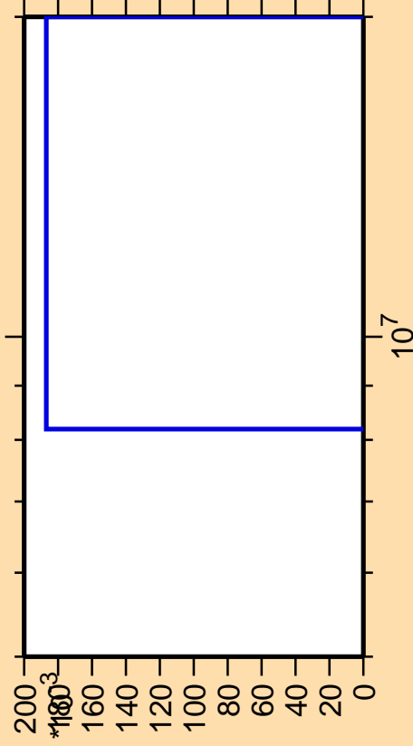
\Delta\sigma/\sigma vs. E for ^{246}\text{Bk}(n,3n\alpha)
