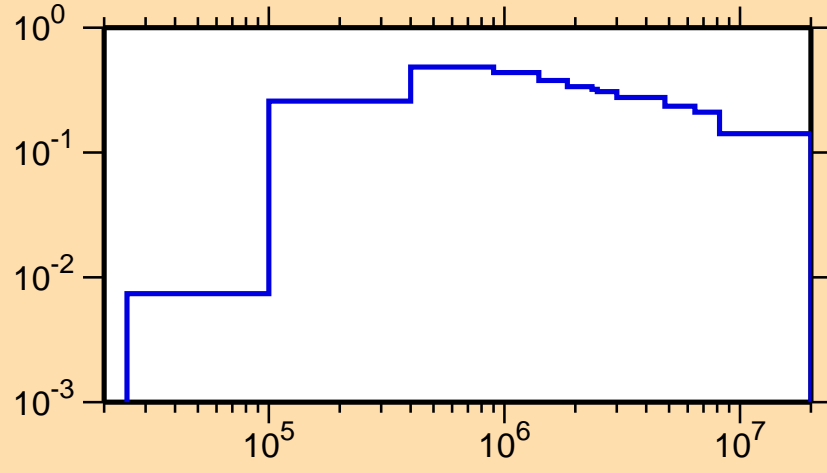
\sigma vs. E for ^{247}\text{Bk}(n,n_3)
