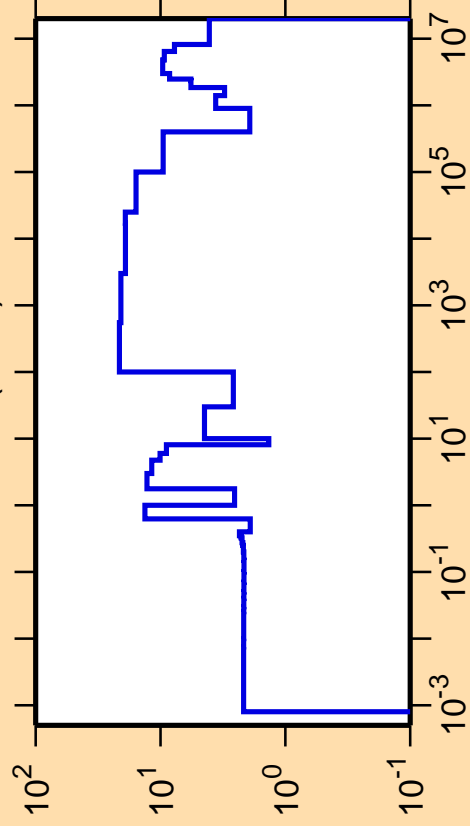
\Delta\sigma/\sigma vs. E for ^{247}\text{Bk}(n,\text{el.})
