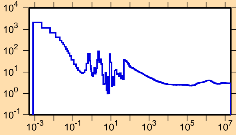
\sigma vs. E for ^{248}\text{Bk}(n,\text{nonel.})
