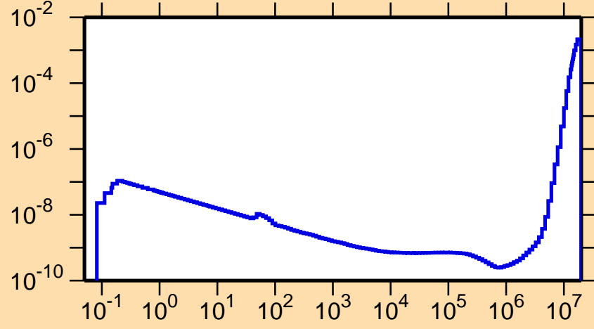
\sigma vs. E for ^{248}\text{Bk}(n,\alpha)
