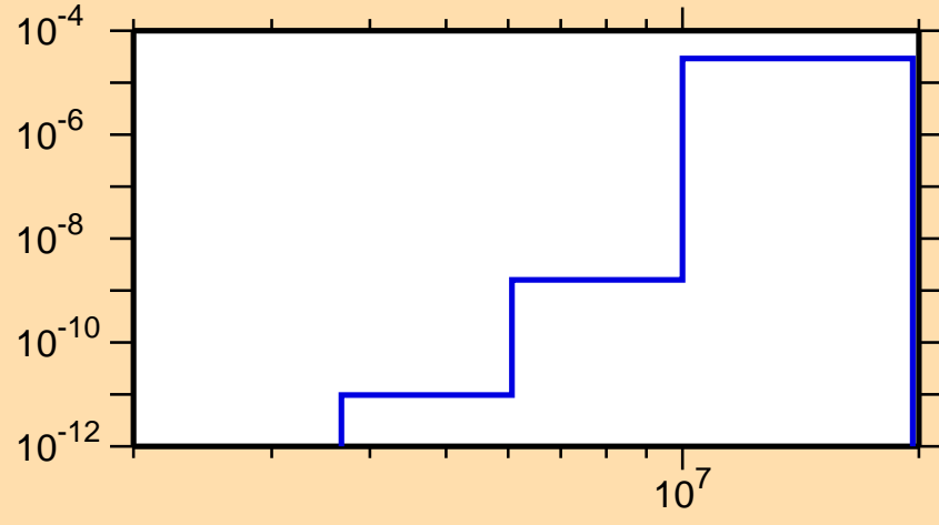
\sigma vs. E for ^{248}\text{Bk}(n,n\alpha)
