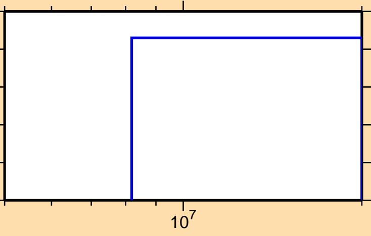
\sigma vs. E for ^{248}\text{Bk}(n,nt)
