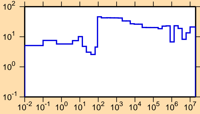
\Delta\sigma/\sigma vs. E for ^{248}\text{Bk}(n,tot.)
