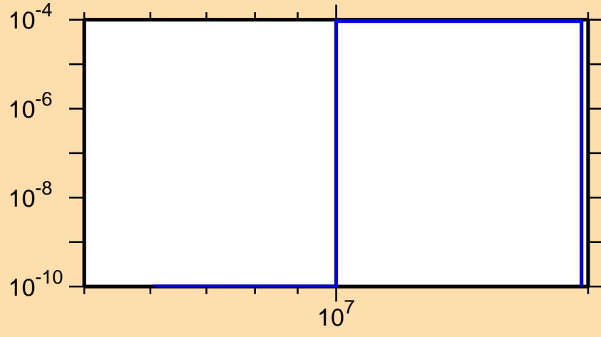
\sigma vs. E for ^{248}\text{Bk}(n,t)
