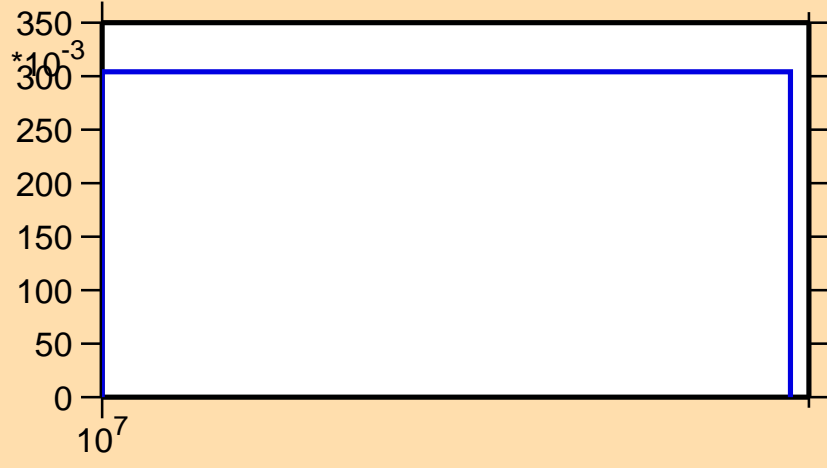
\sigma vs. E for ^{248}\text{Bk}(n,3n)
