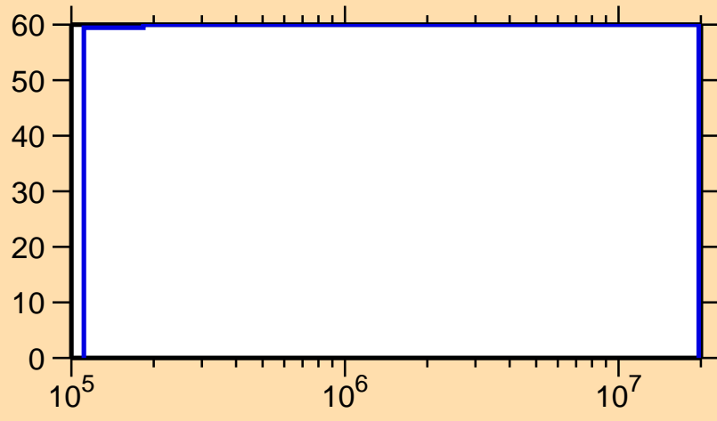
\Delta\sigma/\sigma vs. E for ^{248}\text{Bk}(n,f)
