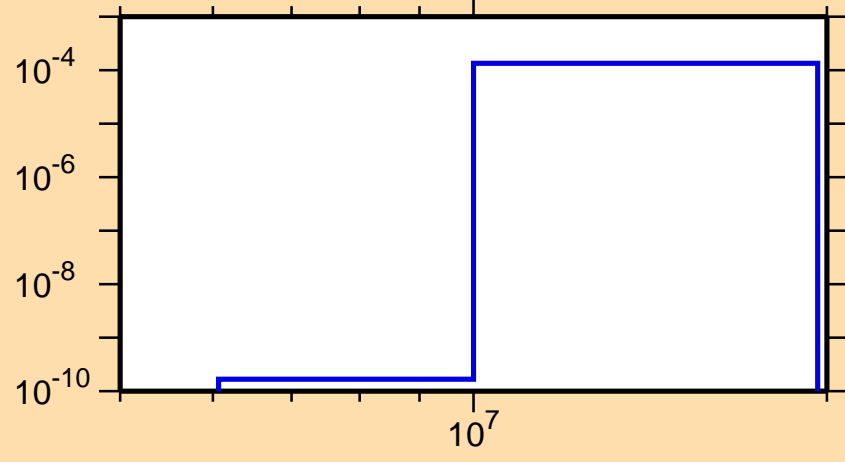
\sigma vs. E for ^{248}\text{Bk}(n,np)
