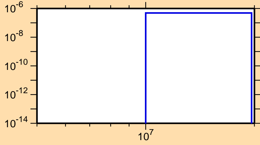
\sigma vs. E for ^{248}\text{Bk}(n,nd)
