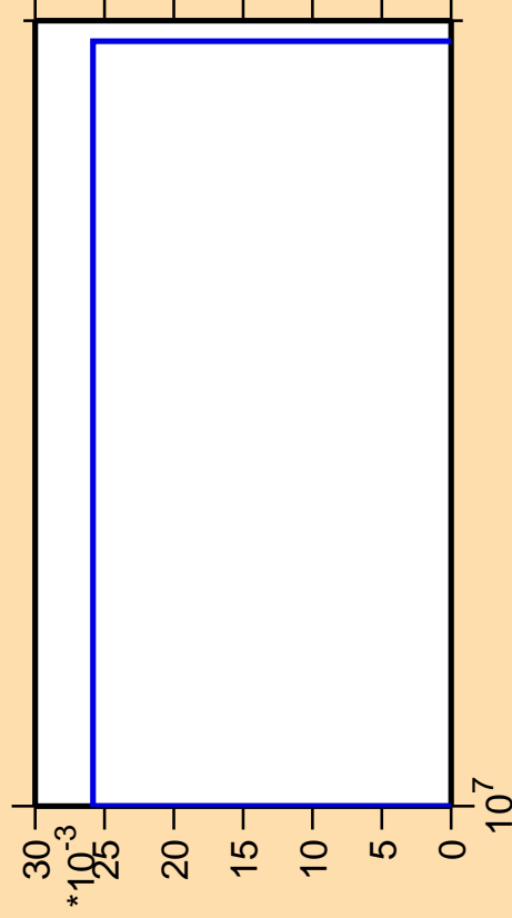
\Delta\sigma/\sigma vs. E for ^{248}\text{Bk} (mt 11)
