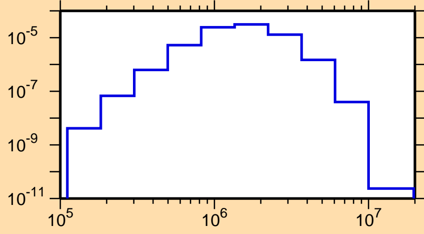
\sigma vs. E for ^{248}\text{Bk}(n,n_2)
