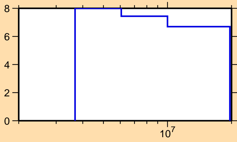
\Delta\sigma/\sigma vs. E for ^{248}\text{Bk}(n,\text{nonel.})
