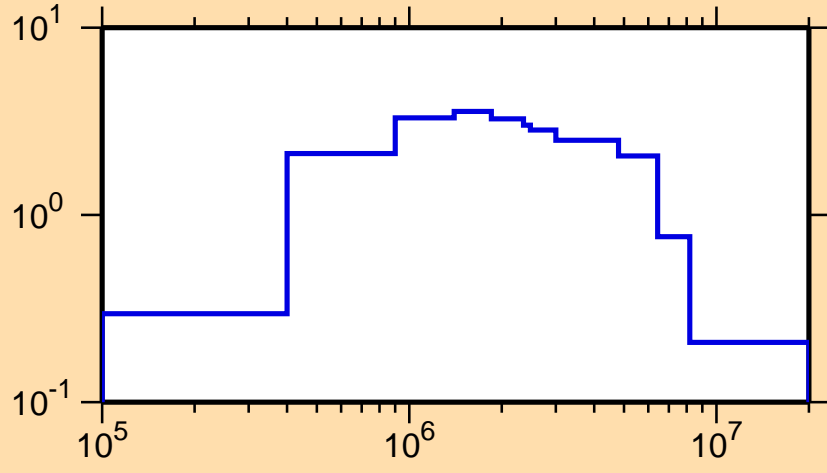
\sigma vs. E for ^{248}\text{Bk}(n,n\text{cont.})
