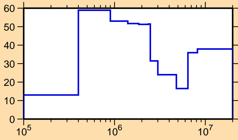
\Delta\sigma/\sigma vs. E for ^{248}\text{Bk}(n,el.)
