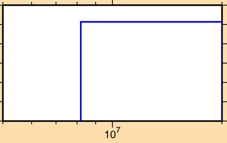
\sigma vs. E for ^{248}\text{Bk}(\text{mt 11})
