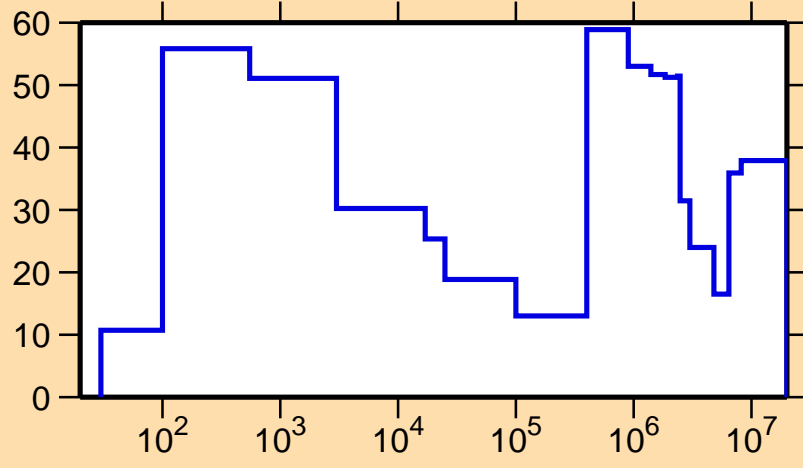
\Delta\sigma/\sigma vs. E for ^{248}\text{Bk}(n,\text{el.})
