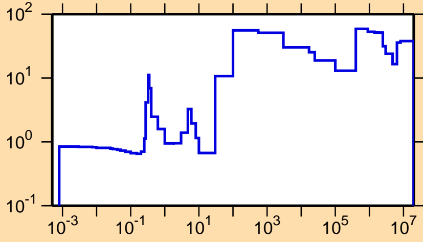
\Delta\sigma/\sigma vs. E for ^{248}\text{Bk}(n,el.)
