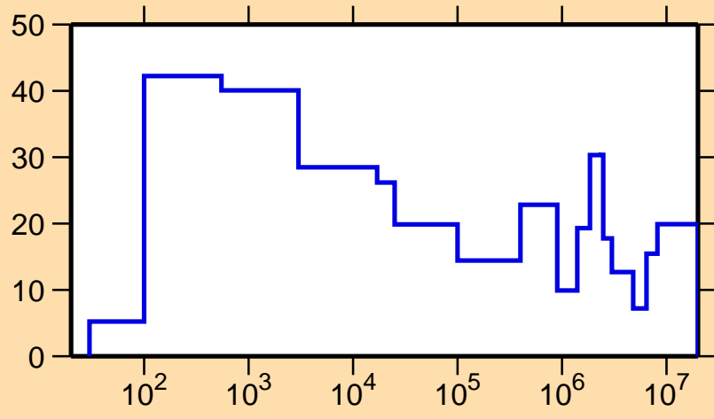
\Delta\sigma/\sigma vs. E for ^{248}\text{Bk}(n,\text{tot.})
