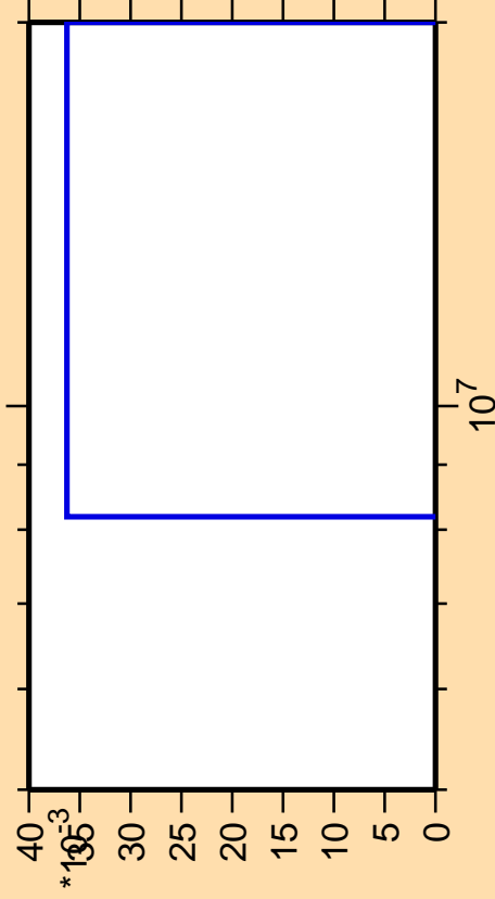
\Delta\sigma/\sigma vs. E for ^{248}\text{Bk}(\text{mt 11})
