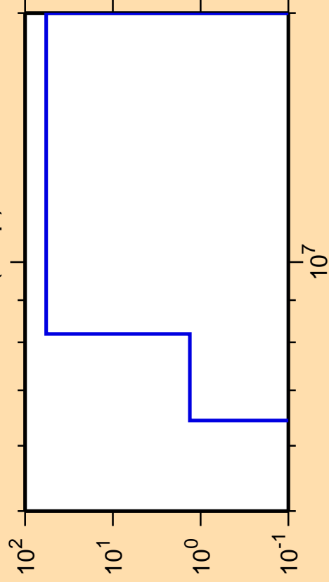
\Delta\sigma/\sigma vs. E for ^{248}\text{Bk}(n,np)
