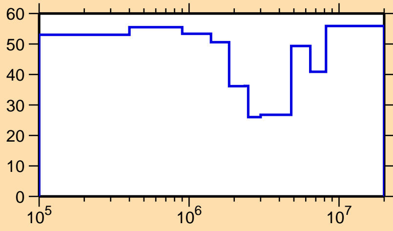
\Delta\sigma/\sigma vs. E for ^{248}\text{Bk}(n,n\text{cont.})
