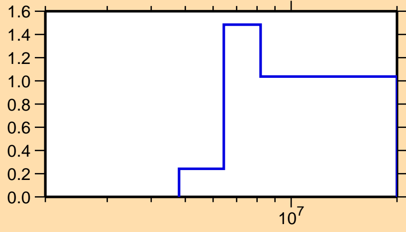
\sigma vs. E for ^{248}\text{Bk}(n,2n)
