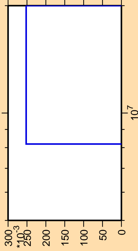
\Delta\sigma/\sigma vs. E for ^{248}\text{Bk}(n,\text{He3})
