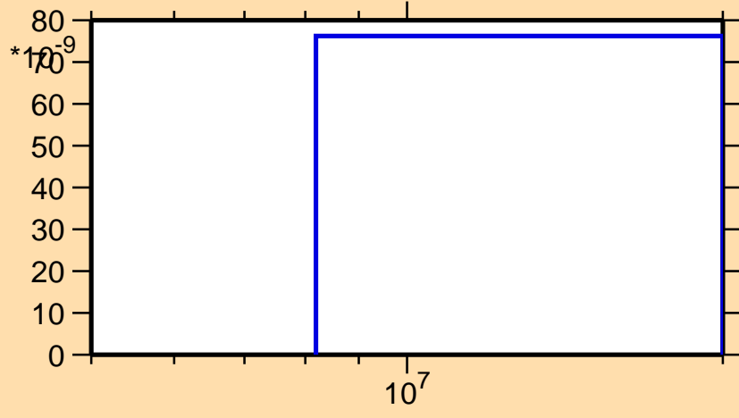
\sigma vs. E for ^{248}\text{Bk}(n,nt)
