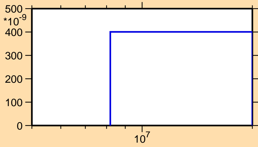
\sigma vs. E for ^{248}\text{Bk}(n,nd)
