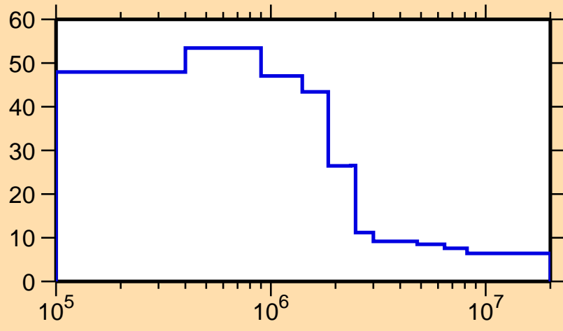
\Delta\sigma/\sigma vs. E for ^{248}\text{Bk}(n,\text{nonel.})
