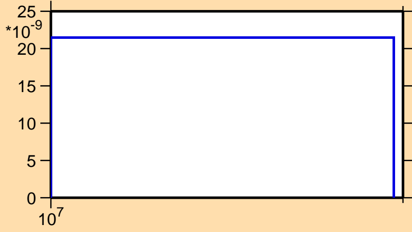
\sigma vs. E for ^{249}\text{Bk}(n,\text{nd})
