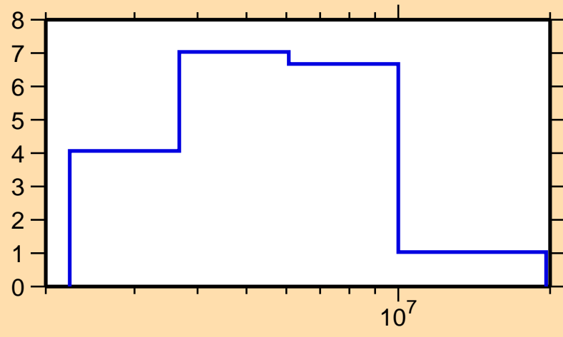
\Delta\sigma/\sigma vs. E for ^{249}\text{Bk}(n,el.)
