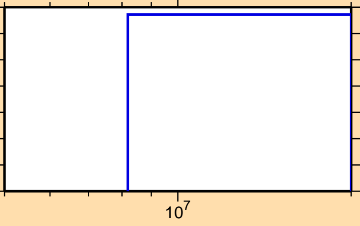
\sigma vs. E for ^{249}\text{Bk}(n,2np)
