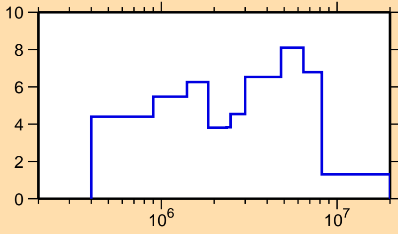
\Delta\sigma/\sigma vs. E for ^{249}\text{Bk}(n,\text{el.})
