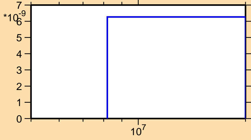
\sigma vs. E for ^{249}\text{Bk}(n,2n\alpha)
