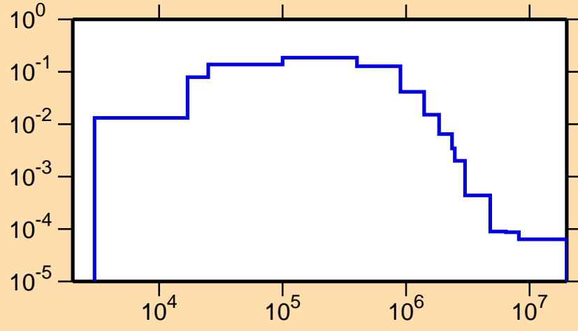
\sigma vs. E for ^{249}\text{Bk}(n,n_1)
