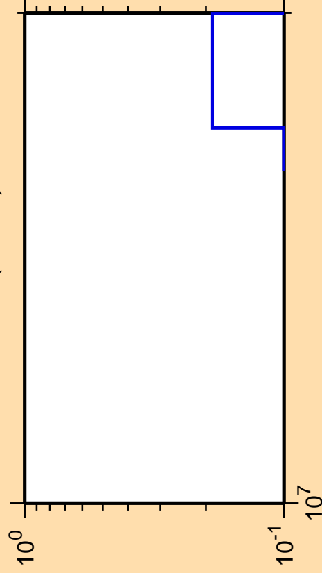
\Delta\sigma/\sigma vs. E for ^{250}\text{Bk} (mt 42)
