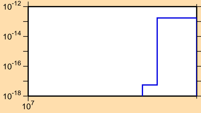
\sigma vs. E for ^{250}\text{Bk} (mt 42)
