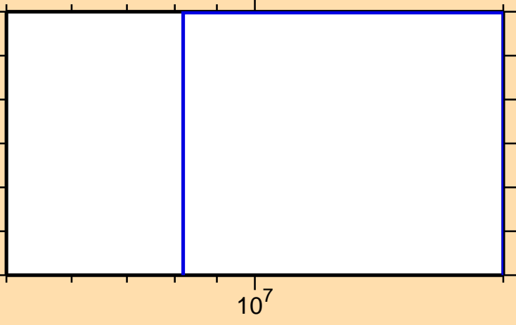
\sigma vs. E for ^{250}\text{Bk}(n,2np)
