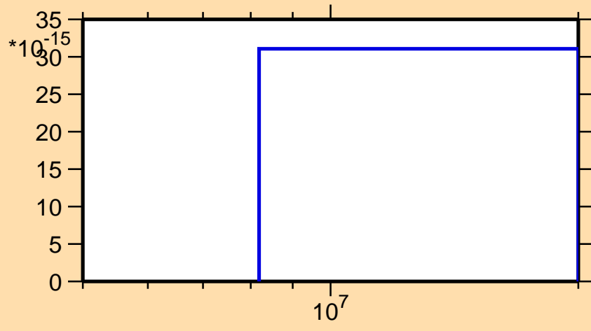
\sigma vs. E for ^{250}\text{Bk}(\text{mt } 11)
