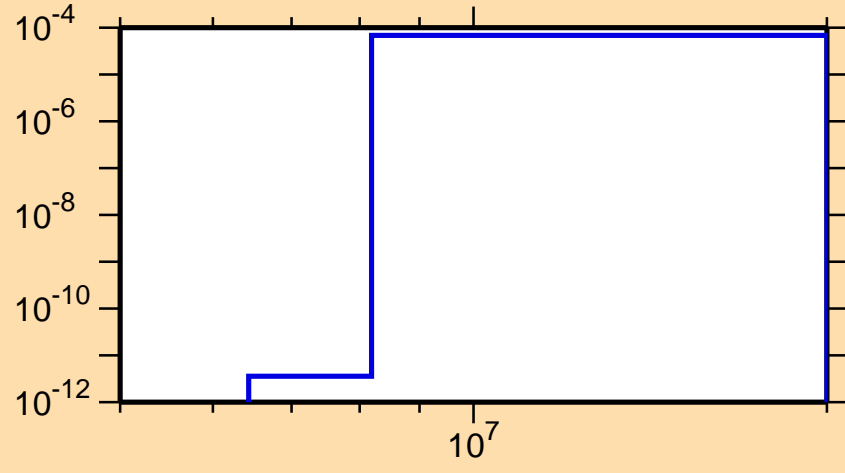
\sigma vs. E for ^{250}\text{Bk}(n,t)
