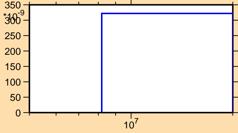
\sigma vs. E for ^{250}\text{Bk}(n,nd)
