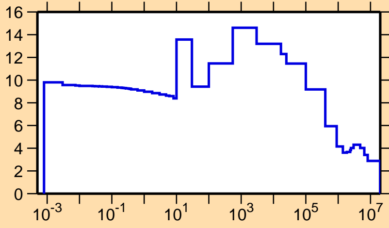
\sigma vs. E for ^{251}\text{Bk}(n,\text{el.})
