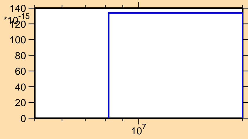
\sigma vs. E for ^{251}\text{Bk}(\text{mt } 11)
