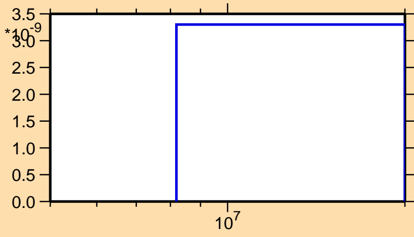
\sigma vs. E for ^{251}\text{Bk}(n,2n\alpha)
