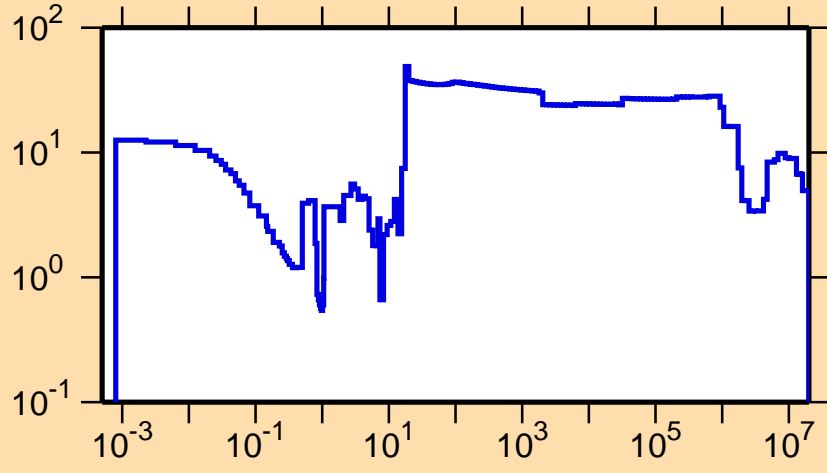
\Delta\sigma/\sigma vs. E for ^{253}\text{Bk}(n,tot.)
