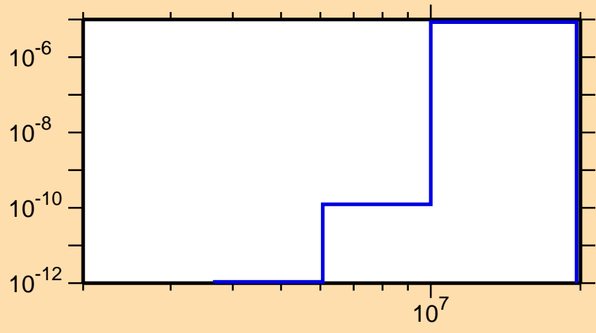
\sigma vs. E for ^{253}\text{Bk}(n,n\alpha)
