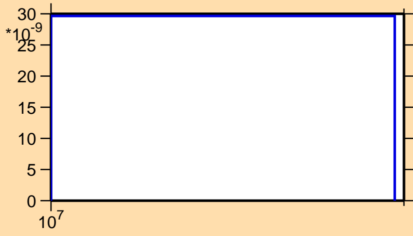
\sigma vs. E for ^{253}\text{Bk}(n,\text{nd})
