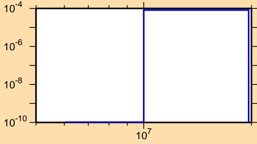
\sigma vs. E for ^{253}\text{Bk}(n,d)
