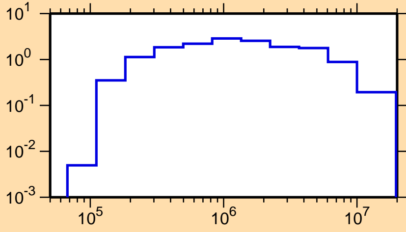
\sigma vs. E for ^{253}\text{Bk}(n,\text{inel.})
