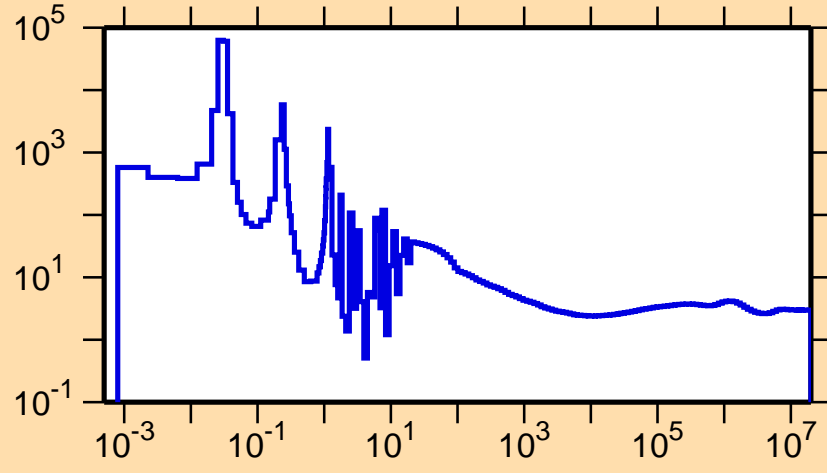
\sigma vs. E for ^{254}\text{Bk}(n,\text{nonel.})
