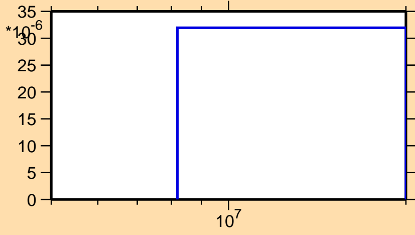
\sigma vs. E for ^{254}\text{Bk}(n,t)
