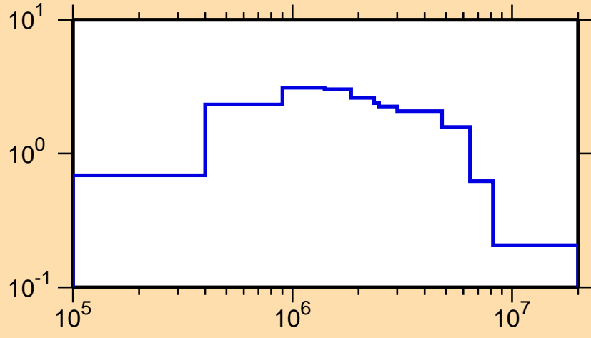
\sigma vs. E for ^{254}\text{Bk}(n,n\text{cont.})
