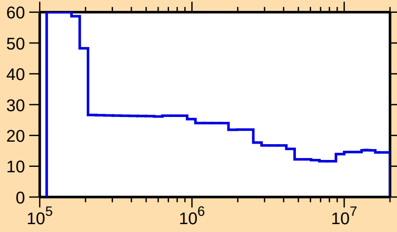
\Delta\sigma/\sigma vs. E for ^{72}\text{Br}(\text{n},\text{nonel.})
