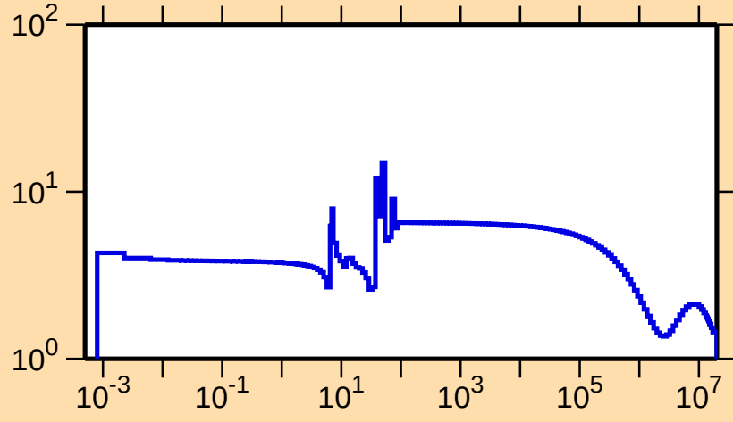
\sigma vs. E for ^{72}\text{Br}(n,\text{el.})
