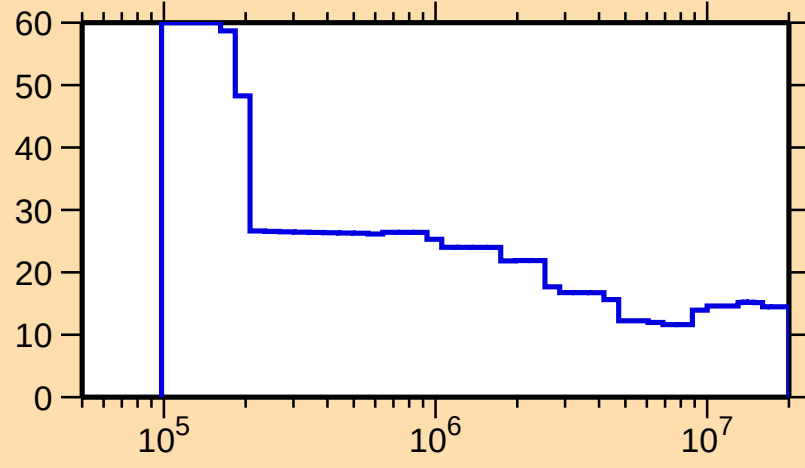
\Delta\sigma/\sigma vs. E for ^{72}\text{Br}(\text{n,nonel.})
