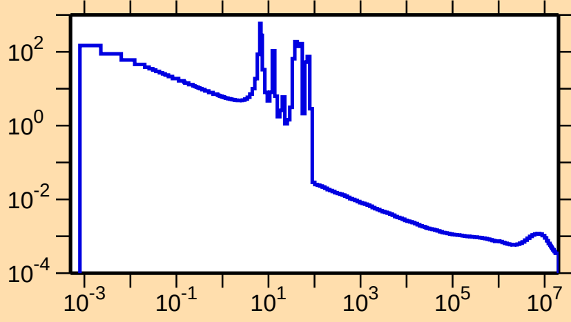
\sigma vs. E for ^{72}\text{Br}(n,\gamma)
