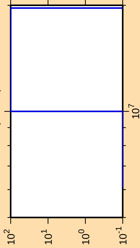
\Delta\sigma/\sigma vs. E for ^{72}\text{Br}(\text{mt } 45)
