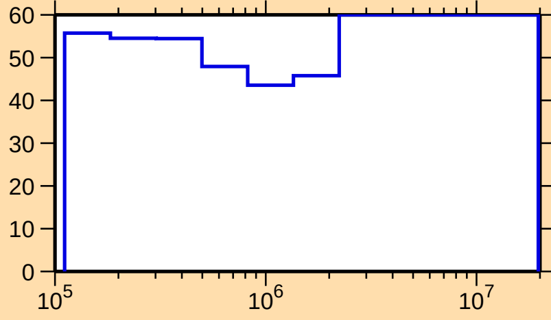
\Delta\sigma/\sigma vs. E for ^{72}\text{Br}(n,n_1)
