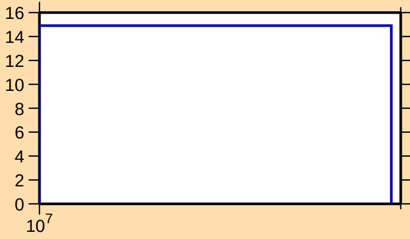
\Delta\sigma/\sigma vs. E for ^{72}\text{Br}(n,\text{nonel.})
