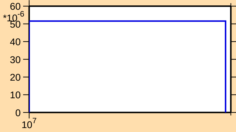
\sigma vs. E for ^{72}\text{Br}(n,2np)
