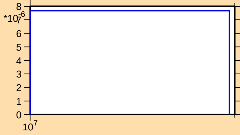
\sigma vs. E for ^{72}\text{Br}(n,\text{pt})
