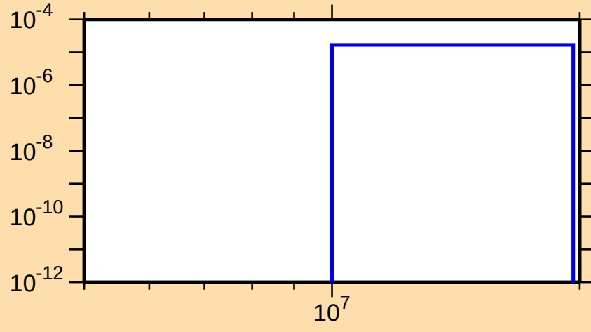
\sigma vs. E for ^{72}\text{Br}(\text{mt } 45)
