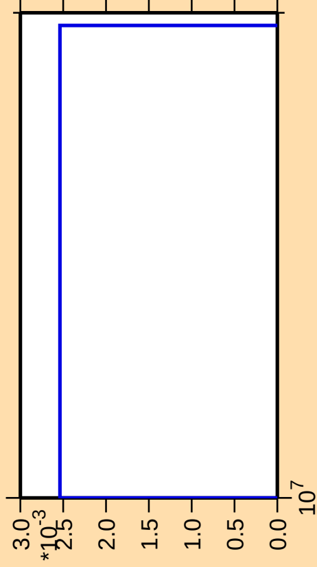
\Delta\sigma/\sigma vs. E for ^{72}\text{Br}(n,\text{nt})
