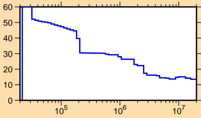
\Delta\sigma/\sigma vs. E for ^{72}\text{Br}(n,n\text{onel.})
