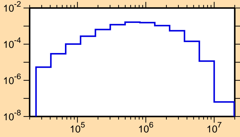
\sigma vs. E for ^{72}\text{Br}(n,n_2)
