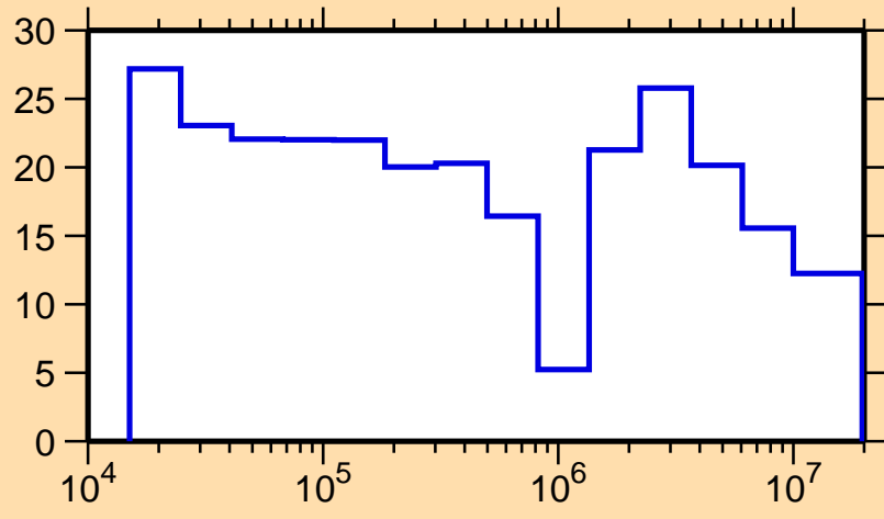
\Delta\sigma/\sigma vs. E for ^{72}\text{Br}(n,el.)
