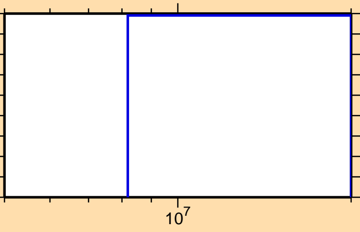
\sigma vs. E for ^{72}\text{Br}(n,2n\alpha)
