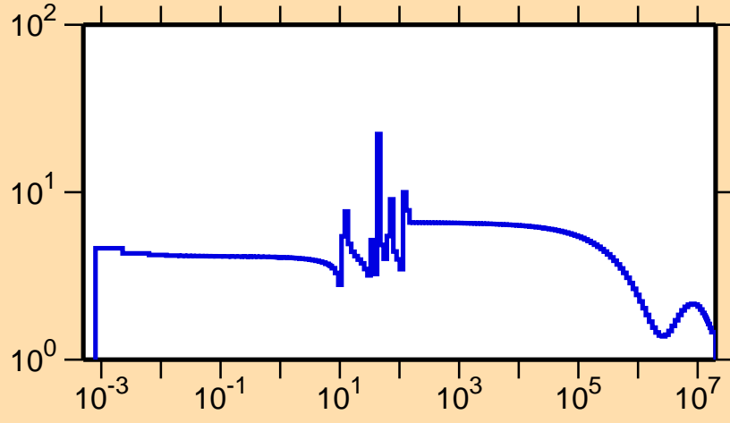
\sigma vs. E for ^{73}\text{Br}(n,\text{el.})
