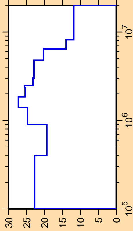
\Delta\sigma/\sigma vs. E for ^{73}\text{Br}(n,n_2)
