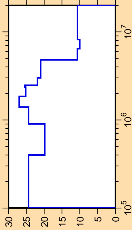
\Delta\sigma/\sigma vs. E for ^{73}\text{Br}(n,n_3)
