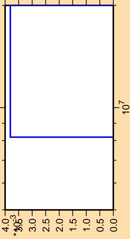
\Delta\sigma/\sigma vs. E for ^{73}\text{Br}(n,2n\alpha)
