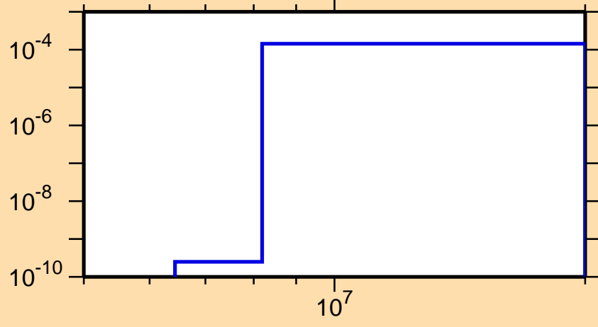
\sigma vs. E for ^{73}\text{Br}(n,\text{He3})
