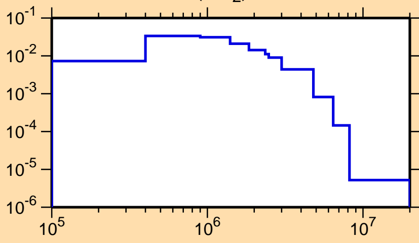
\sigma vs. E for ^{73}\text{Br}(n,n_2)
