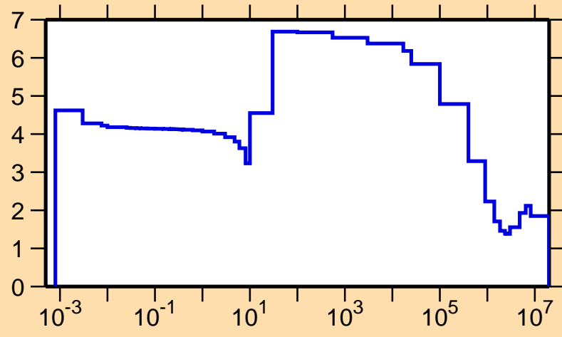
\sigma vs. E for ^{73}\text{Br}(n,\text{el.})
