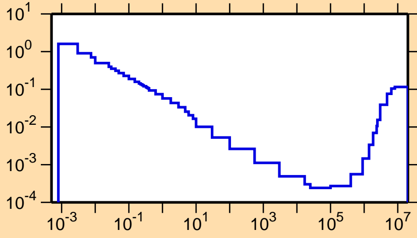
\sigma vs. E for ^{73}\text{Br}(n,\alpha)
