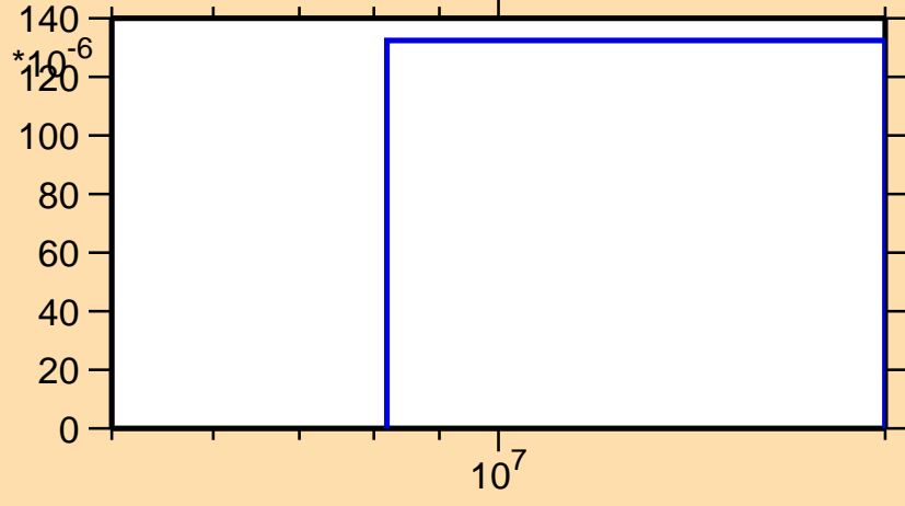
\sigma vs. E for ^{73}\text{Br}(n,t)
