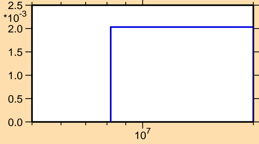
\sigma vs. E for ^{73}\text{Br}(n,2n)
