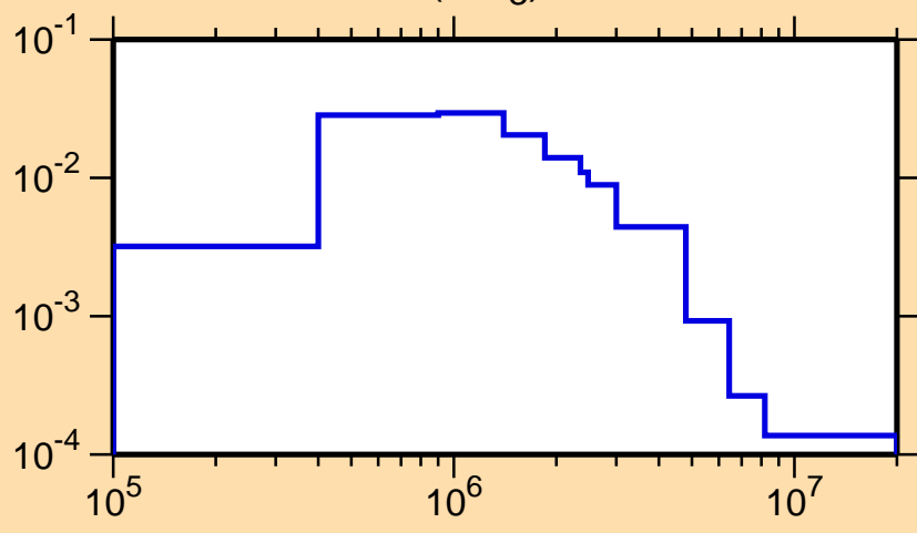
\sigma vs. E for ^{73}\text{Br}(n,n_3)
