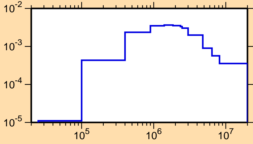
\sigma vs. E for ^{74}\text{Br}(n,n_2)
