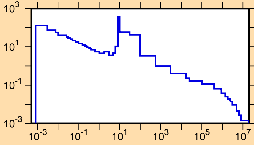
\sigma vs. E for ^{76}\text{Br}(n,\gamma)
