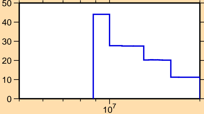
\Delta\sigma/\sigma vs. E for ^{76}\text{Br}(n,2n)
