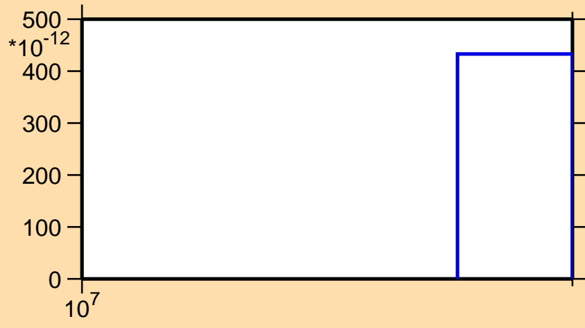
\sigma vs. E for ^{76}\text{Br}(n,nt)
