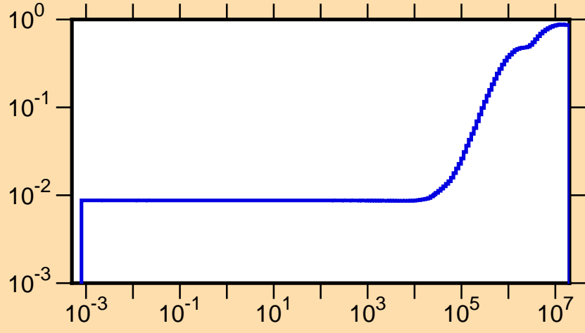
\mu vs. E for ^{77}\text{Br}(\text{mt251})
