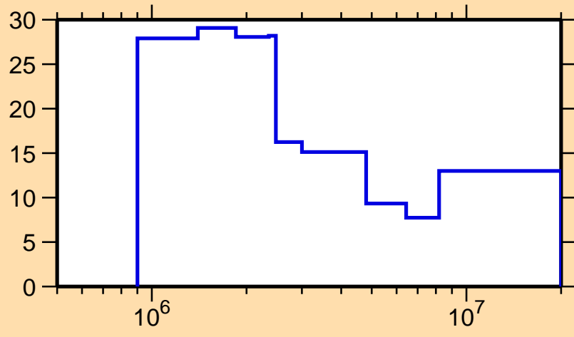
\Delta\sigma/\sigma vs. E for ^{77}\text{Br}(n,el.)
