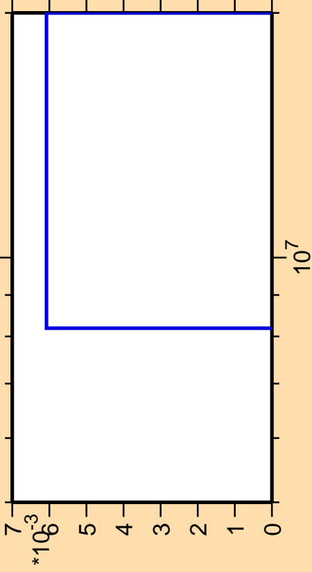
\Delta\sigma/\sigma vs. E for ^{77}\text{Br}(n,2n\alpha)
