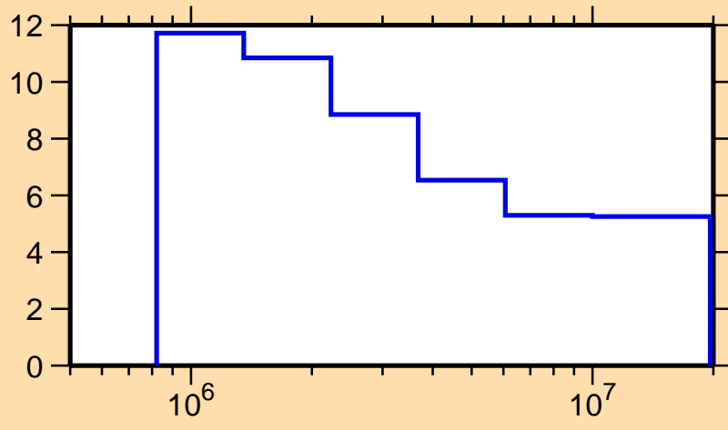
\Delta\sigma/\sigma vs. E for ^{79}\text{Br}(n,n\text{onel.})
