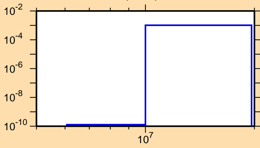
\sigma vs. E for ^{79}\text{Br}(n,n\alpha)
