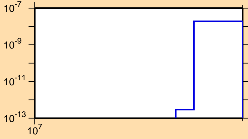
\sigma vs. E for ^{80}\text{Br}(n,2n\alpha)
