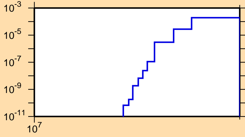
\sigma vs. E for ^{80}\text{Br}(n,nd)
