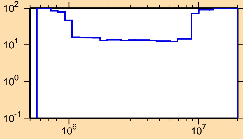
\Delta\sigma/\sigma vs. E for ^{80}\text{Br}(n,n\text{cont.})
