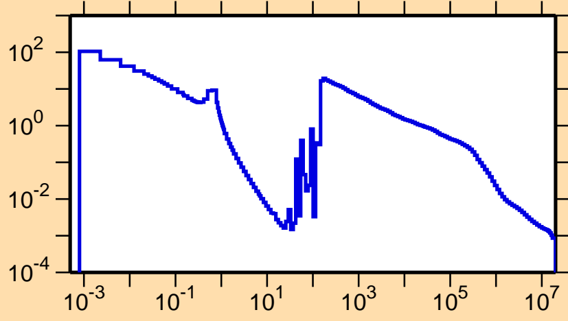
\sigma vs. E for ^{80}\text{Br}(n,\gamma)
