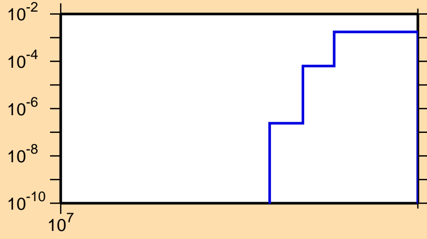
\sigma vs. E for ^{80}\text{Br}(n,2np)
