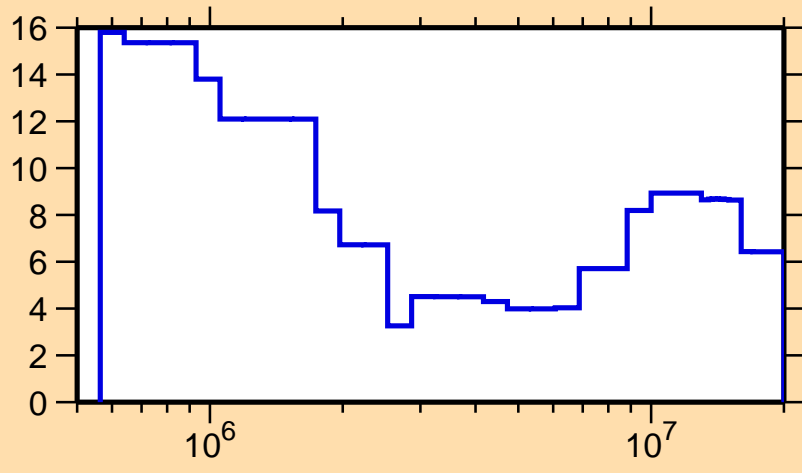
\Delta\sigma/\sigma vs. E for ^{80}\text{Br}(n,\text{tot.})
