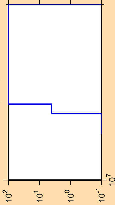
\Delta\sigma/\sigma vs. E for ^{80}\text{Br}(n,nd)
