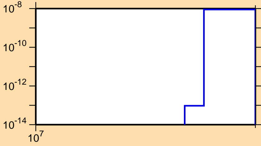
\sigma vs. E for ^{80}\text{Br}(n,nt)
