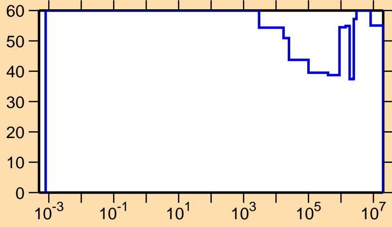
\Delta\sigma/\sigma vs. E for ^{80}\text{Br}(n,p)
