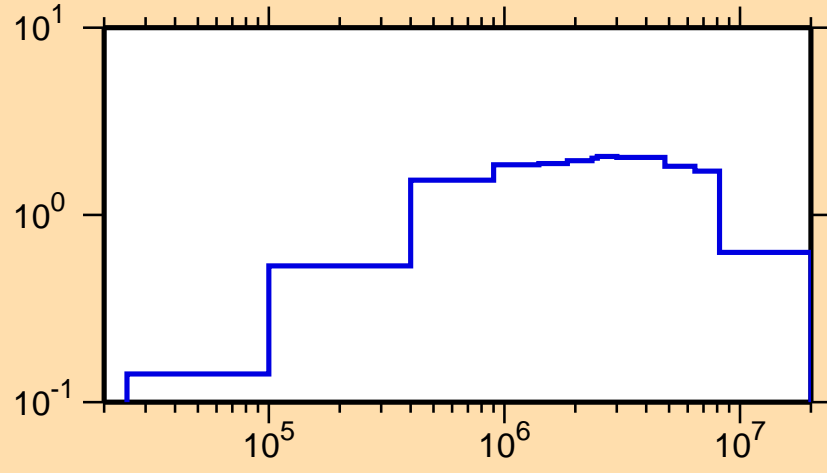
\sigma vs. E for ^{80}\text{Br}(n,\text{inel.})
