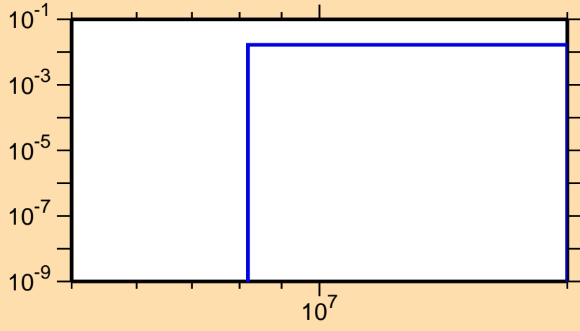
\sigma vs. E for ^{80}\text{Br}(n,np)
