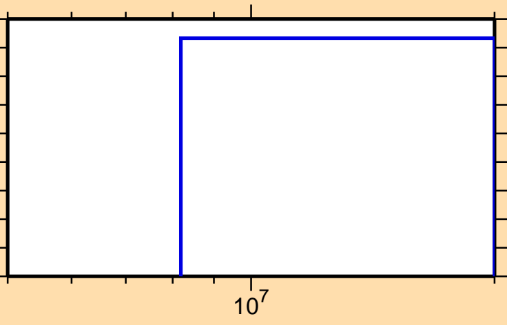
\sigma vs. E for ^{80}\text{Br}(n,2np)
