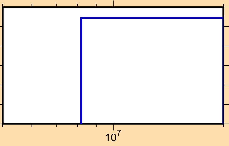
\sigma vs. E for ^{80}\text{Br}(n,\text{He}3)
