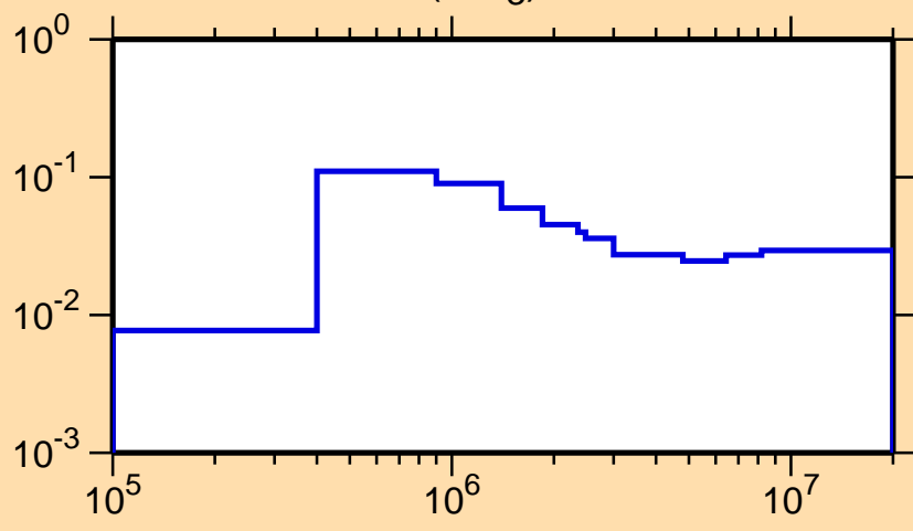
\sigma vs. E for ^{82}\text{Br}(n,n_3)
