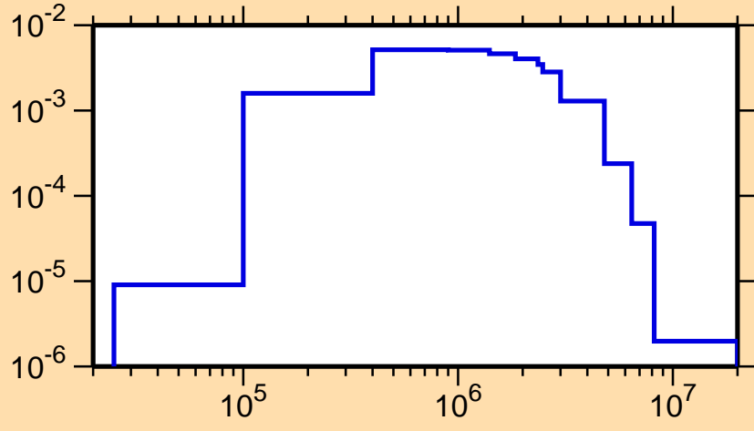
\sigma vs. E for ^{82}\text{Br}(n,n_2)
