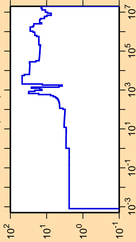
\Delta\sigma/\sigma vs. E for ^{83}\text{Br}(n,\text{el.})
