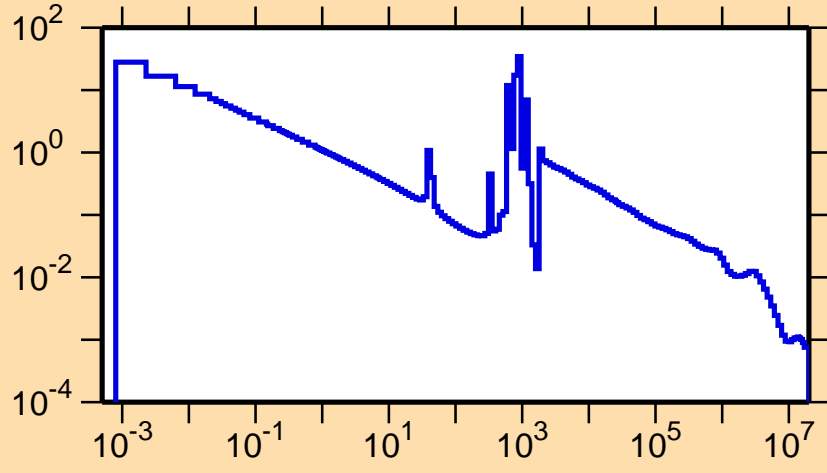
\sigma vs. E for ^{83}\text{Br}(n,\gamma)
