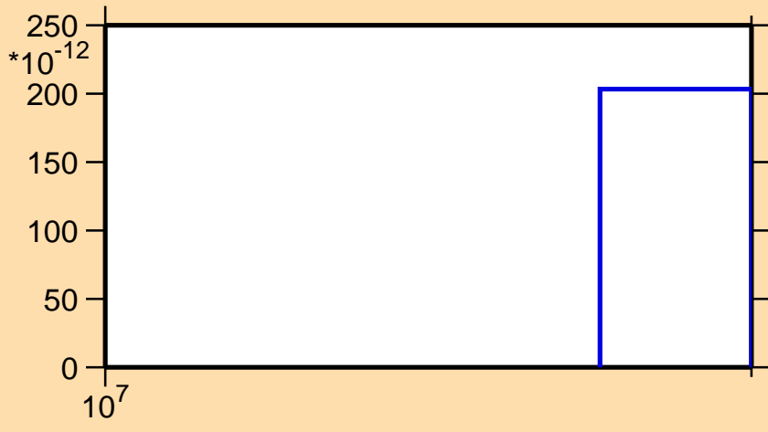
\sigma vs. E for ^{83}\text{Br}(n,2np)
