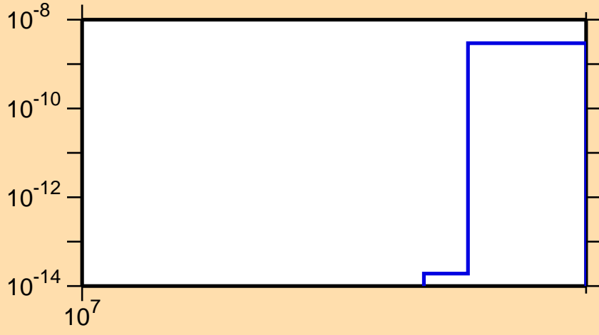
\sigma vs. E for ^{83}\text{Br}(n,nt)
