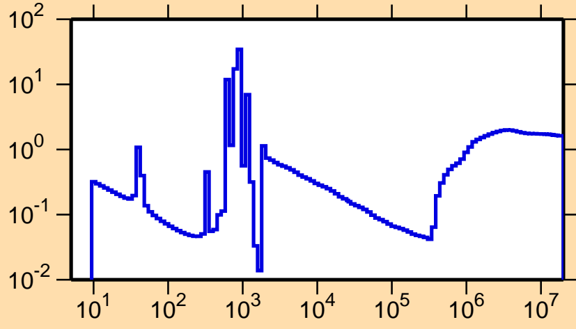
\sigma vs. E for ^{83}\text{Br}(n,\text{nonel.})
