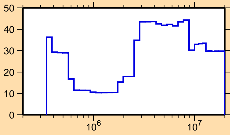
\Delta\sigma/\sigma vs. E for ^{83}\text{Br}(n,n_1)
