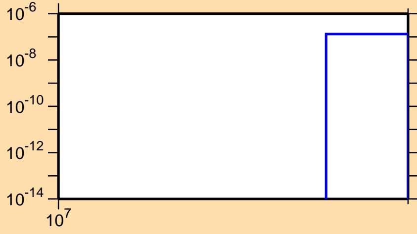
\sigma vs. E for ^{83}\text{Br}(n,\text{nd})
