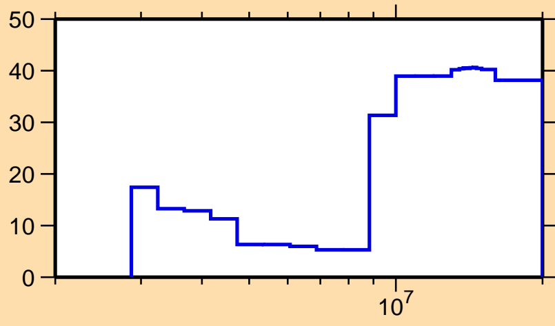
\Delta\sigma/\sigma vs. E for ^{83}\text{Br}(n,ncont.)
