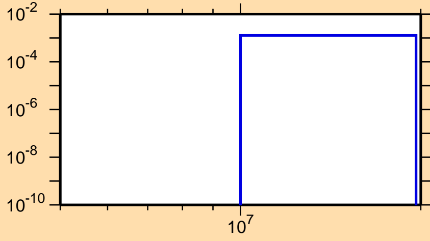
\sigma vs. E for ^{83}\text{Br}(n,np)
