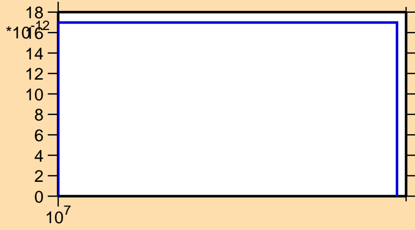
\sigma vs. E for ^{83}\text{Br}(n,nt)
