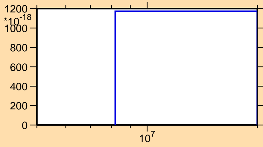
\sigma vs. E for ^{83}\text{Br}(n,\text{He}3)
