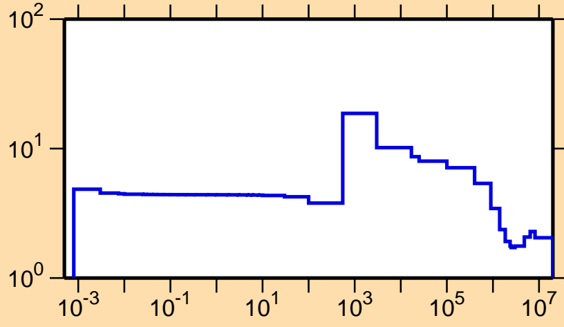
\sigma vs. E for ^{83}\text{Br}(n,\text{el.})
