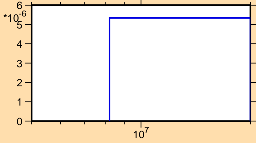
\sigma vs. E for ^{83}\text{Br}(n,t)
