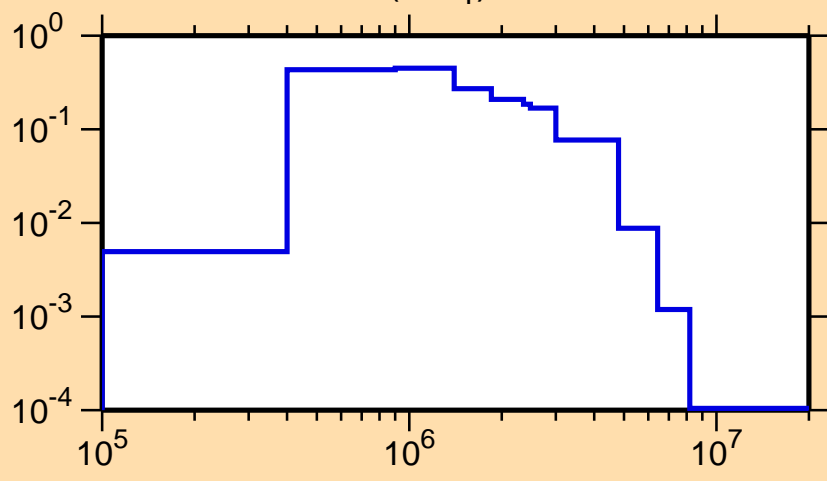
\sigma vs. E for ^{83}\text{Br}(n,n_1)
