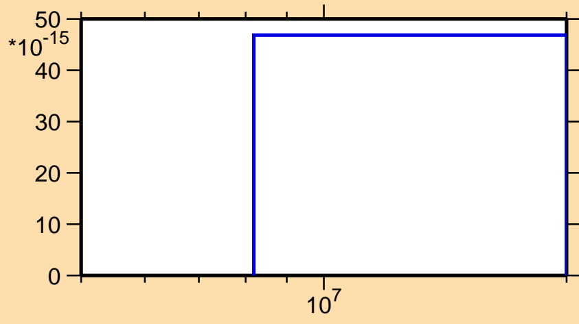
\sigma vs. E for ^{84}\text{Br}(n,2n\alpha)
