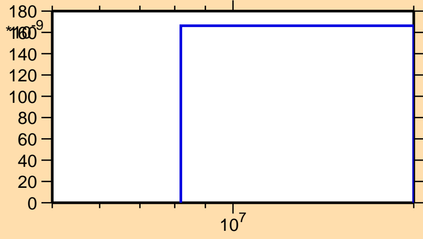
\sigma vs. E for ^{87}\text{Br}(n,nt)
