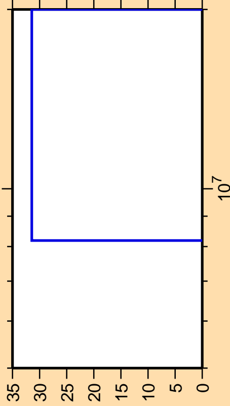
\Delta\sigma/\sigma vs. E for ^{87}\text{Br}(n,3n)
