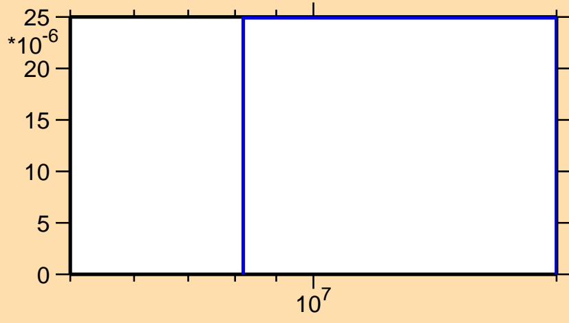
\sigma vs. E for ^{87}\text{Br}(n,t)
