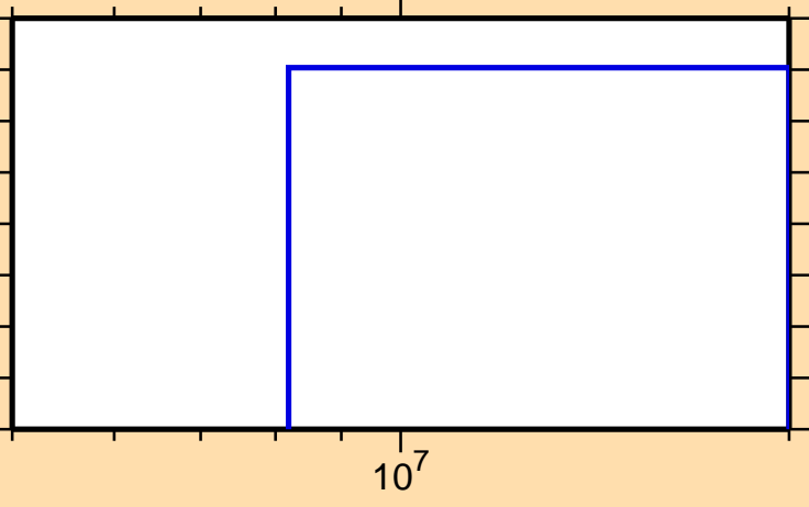
\sigma vs. E for ^{87}\text{Br}(n,\text{nd})
