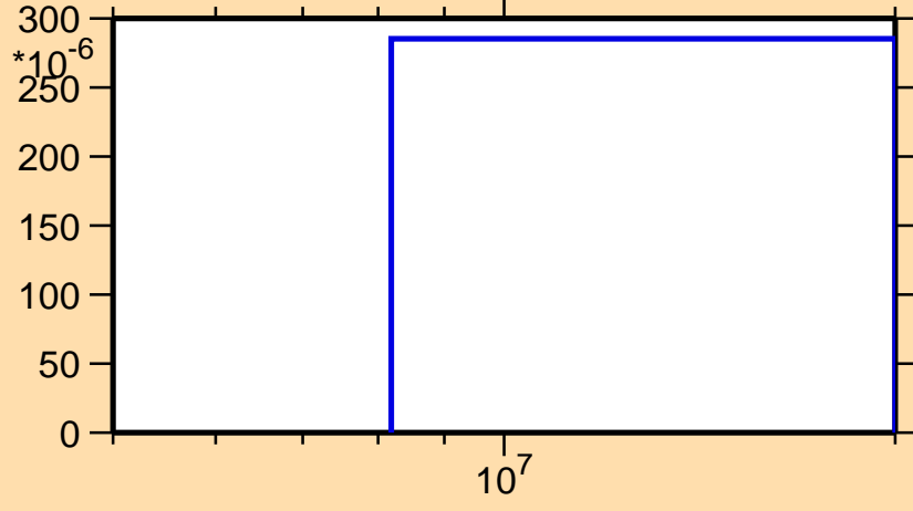
\sigma vs. E for ^{87}\text{Br}(n,d)
