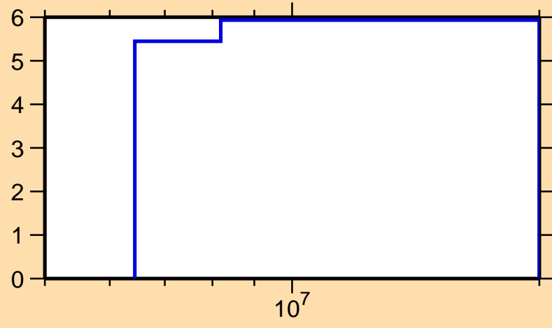
\Delta\sigma/\sigma vs. E for ^{87}\text{Br}(n,\text{nonel.})
