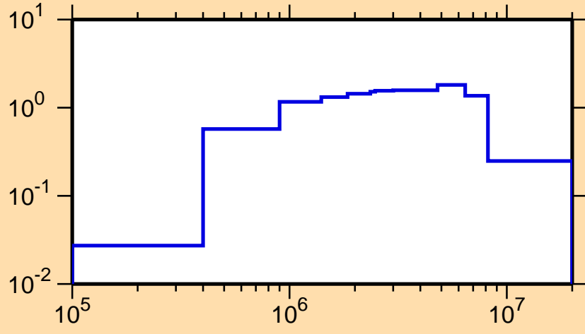
\sigma vs. E for ^{87}\text{Br}(n,\text{inel.})
