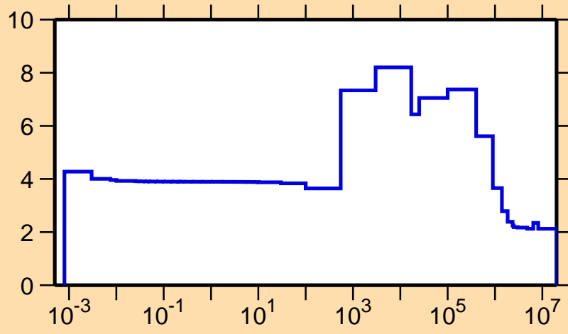
\sigma vs. E for ^{87}\text{Br}(n,\text{el.})
