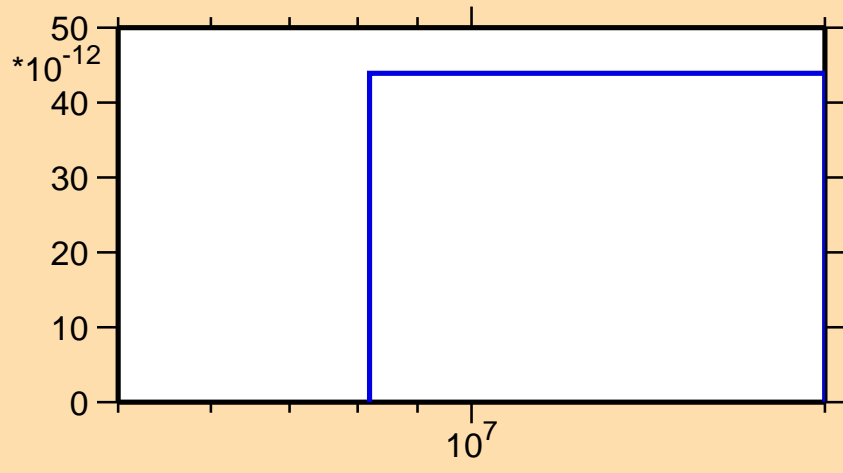
\sigma vs. E for ^{87}\text{Br}(n,2np)
