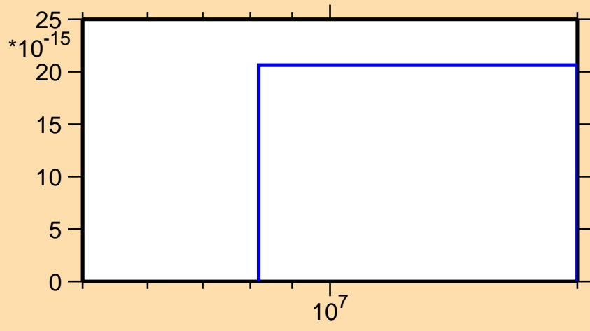
\sigma vs. E for ^{87}\text{Br}(n,2n\alpha)
