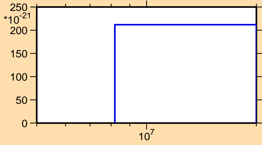
\sigma vs. E for ^{88}\text{Br}(\text{mt } 11)
