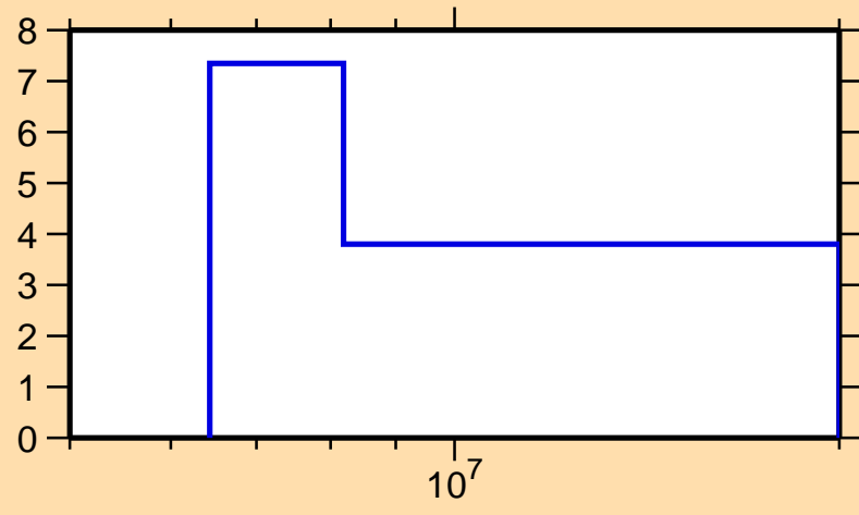
\Delta\sigma/\sigma vs. E for ^{88}\text{Br}(n,\text{nonel.})
