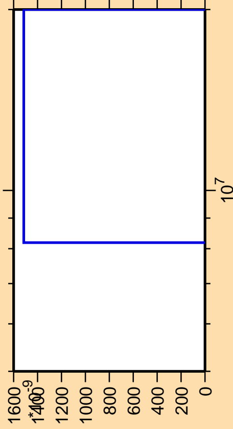
\Delta\sigma/\sigma vs. E for ^{88}\text{Br}(\text{mt } 11)
