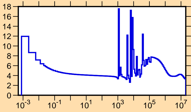
\sigma vs. E for ^{89}\text{Br}(n,\text{tot.})
