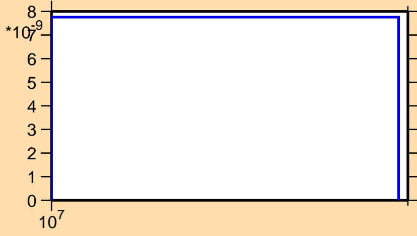
\sigma vs. E for ^{89}\text{Br}(n,\text{nd})
