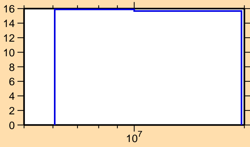
\Delta\sigma/\sigma vs. E for ^{89}\text{Br}(n,\text{nonel.})
