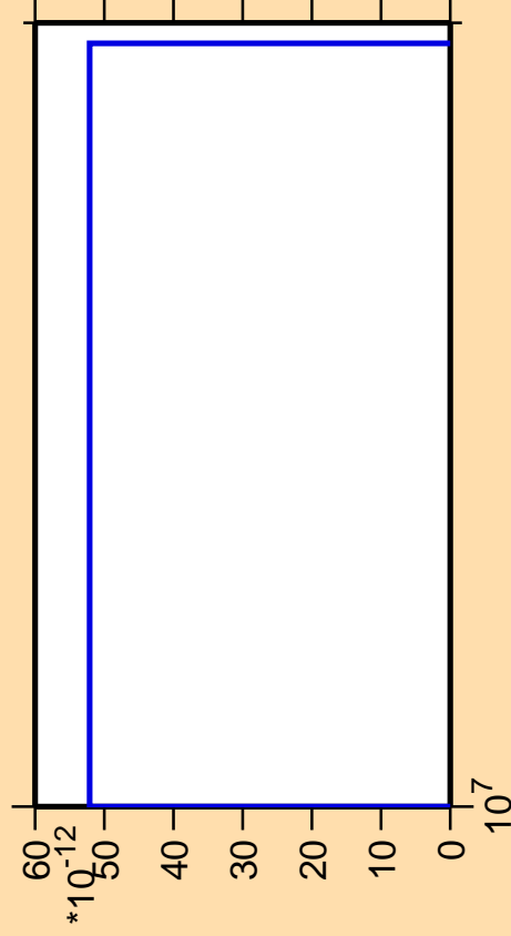
\Delta\sigma/\sigma vs. E for ^{89}\text{Br} (mt 11)
