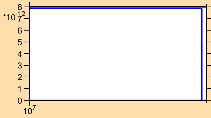
\sigma vs. E for ^{89}\text{Br}(n,2np)
