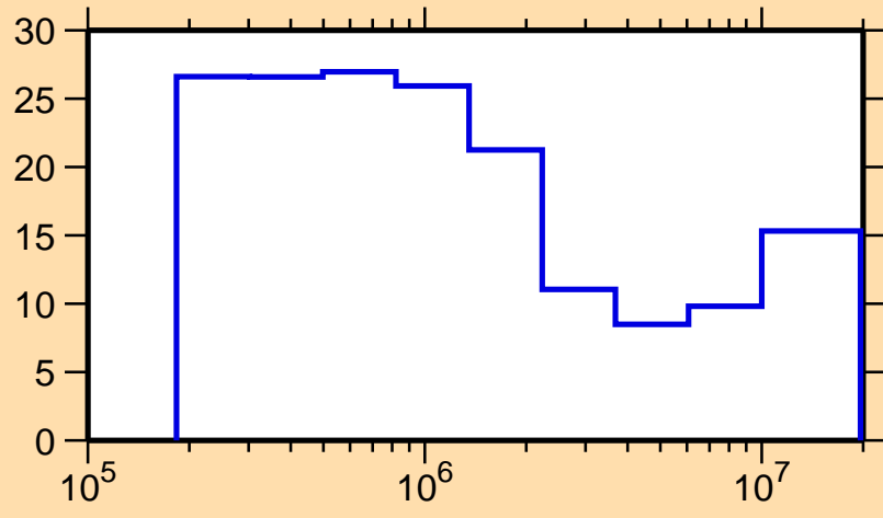
\Delta\sigma/\sigma vs. E for ^{89}\text{Br}(n,\text{tot.})
