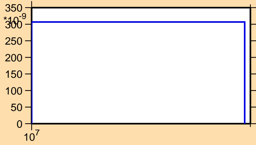
\sigma vs. E for ^{89}\text{Br}(n,nt)
