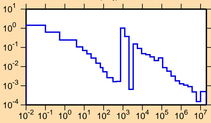
\sigma vs. E for ^{89}\text{Br}(n,\gamma)
