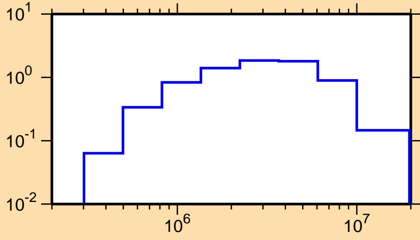
\sigma vs. E for ^{89}\text{Br}(n,n\text{cont.})
