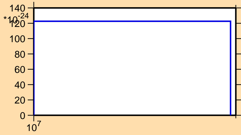
\sigma vs. E for ^{89}\text{Br} (mt 11)
