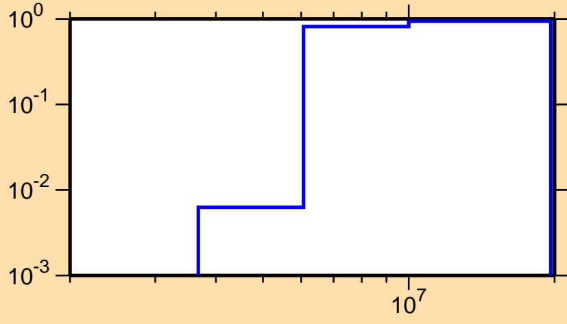
\sigma vs. E for ^{89}\text{Br}(n,2n)
