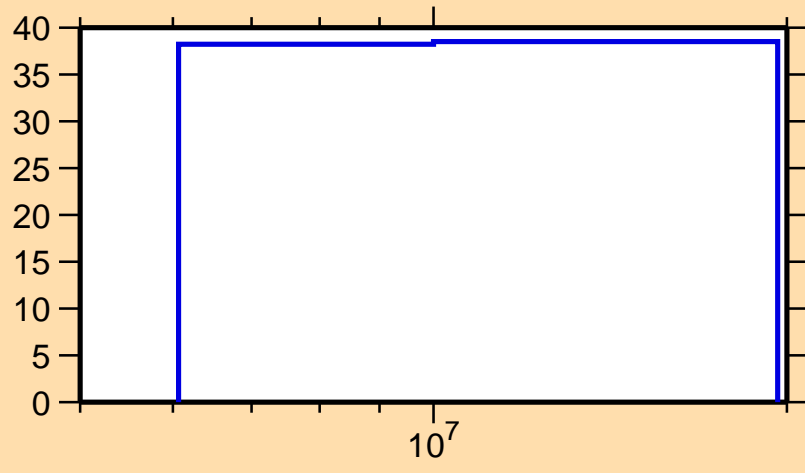
\Delta\sigma/\sigma vs. E for ^{89}\text{Br}(n,2n)
