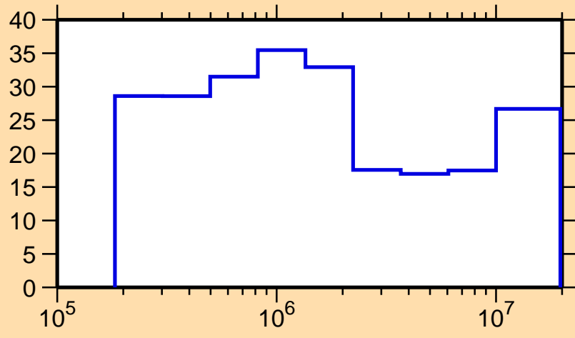
\Delta\sigma/\sigma vs. E for ^{89}\text{Br}(n,\text{el.})
