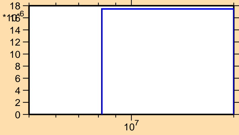
\sigma vs. E for ^{89}\text{Br}(n,t)
