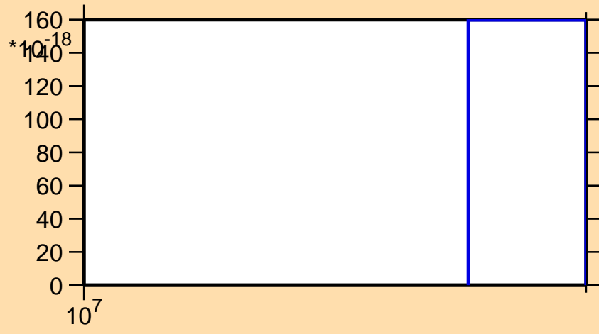
\sigma vs. E for ^{90}\text{Br} (mt 11)
