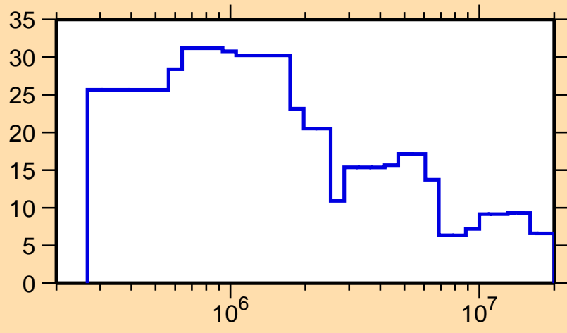
\Delta\sigma/\sigma vs. E for ^{90}\text{Br}(n,\text{tot.})
