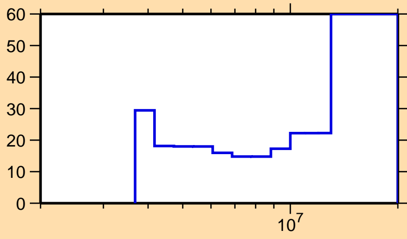
\Delta\sigma/\sigma vs. E for ^{90}\text{Br}(n,2n)
