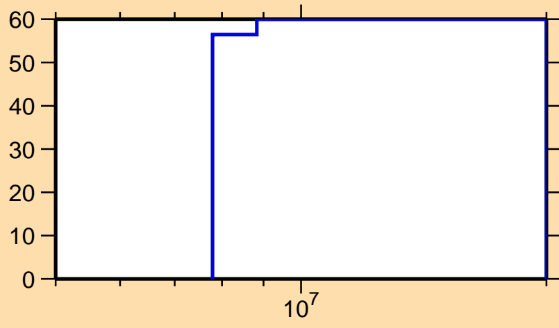
\Delta\sigma/\sigma vs. E for ^{90}\text{Br}(n,p)
