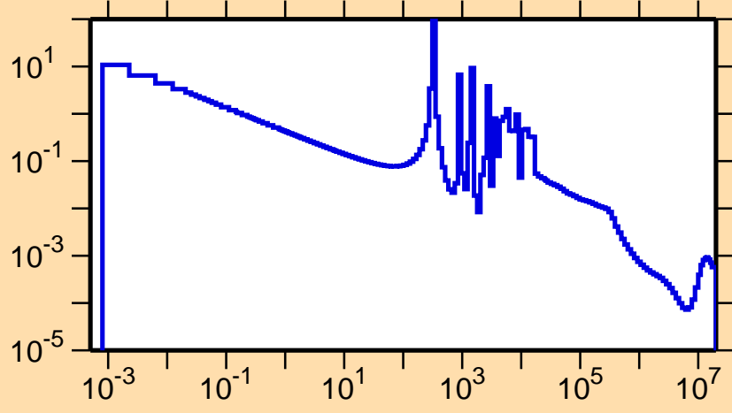
\sigma vs. E for ^{90}\text{Br}(n,\gamma)
