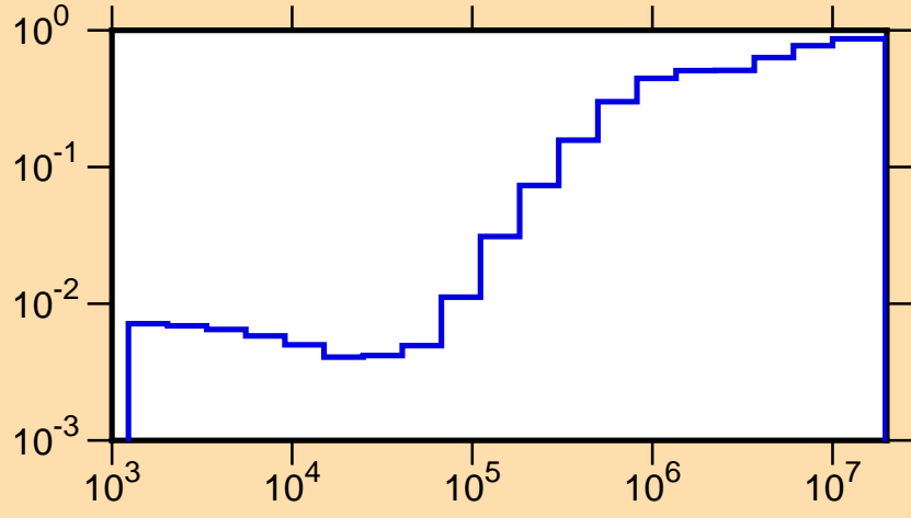
\mu vs. E for ^{90}\text{Br}(\text{mt251})
