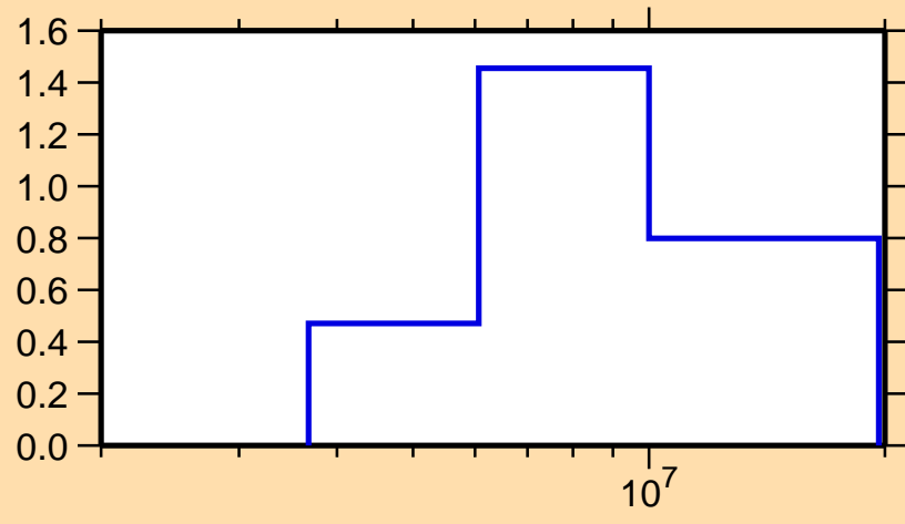
\sigma vs. E for ^{90}\text{Br}(n,2n)
