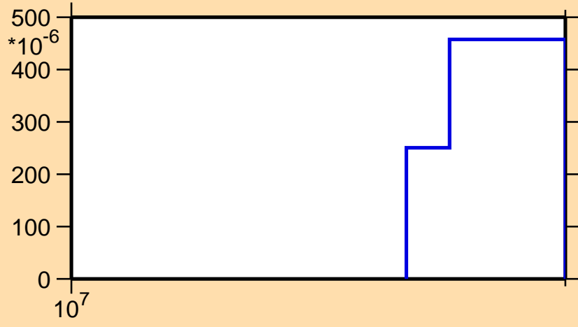
\sigma vs. E for ^{11}\text{C}(n,2n)
