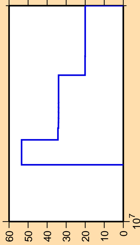
\Delta\sigma/\sigma vs. E for ^{11}\text{C} (mt117)
