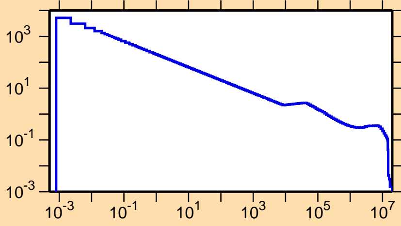
\sigma vs. E for ^{11}\text{C}(n,p)
