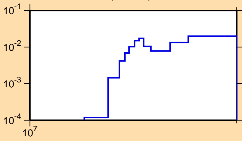
\sigma vs. E for ^{11}\text{C} (mt117)
