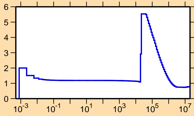
\sigma vs. E for ^{11}\text{C}(n,\text{el.})
