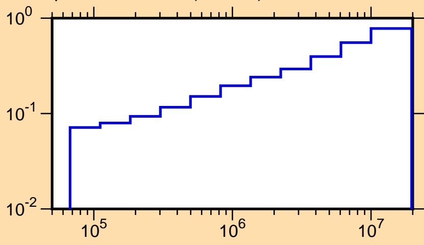
\mu vs. E for ^{11}\text{C} (mt251)
