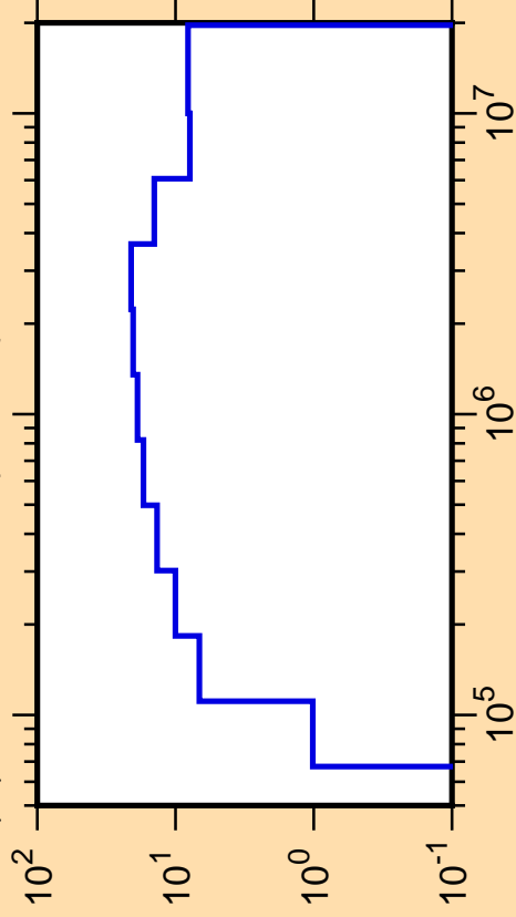
\Delta\mu/\mu vs. E for ^{11}\text{C} (mt251)
